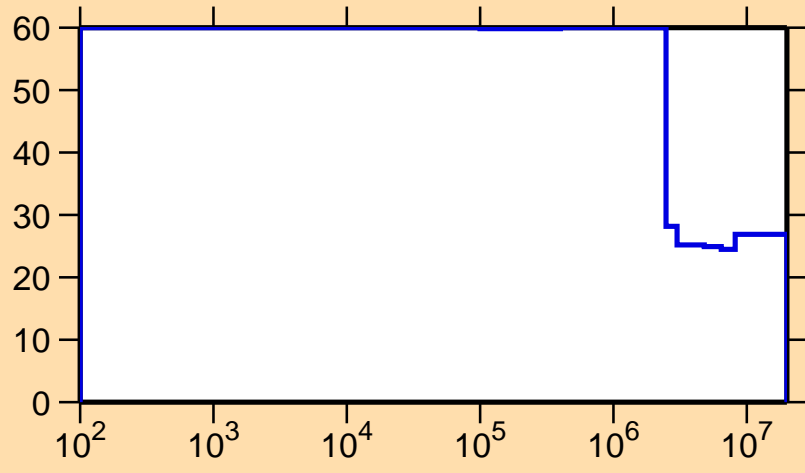
\Delta\sigma/\sigma vs. E for ^{258}\text{Lw}(n,p)
