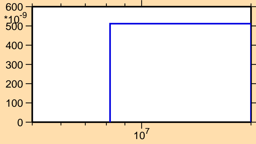
\sigma vs. E for ^{258}\text{Lw}(n,nd)
