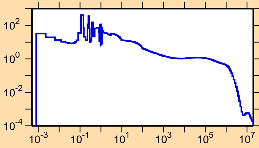
\sigma vs. E for ^{259}\text{Lw}(n,\gamma)
