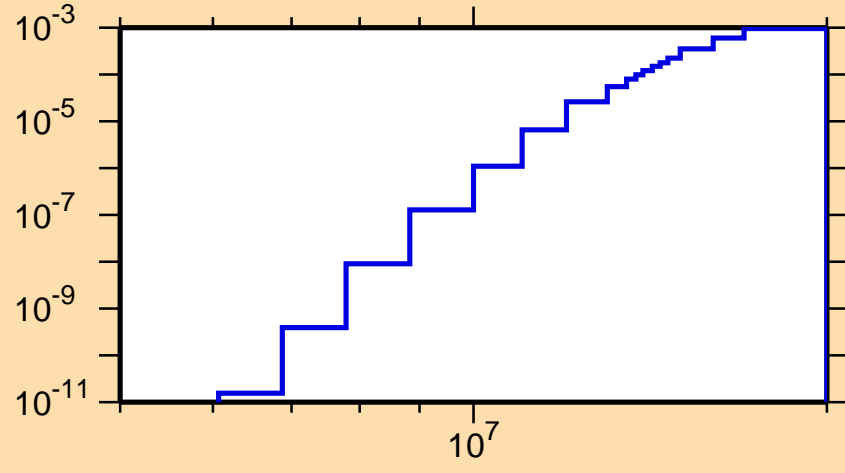
\sigma vs. E for ^{259}\text{Lw}(n,d)
