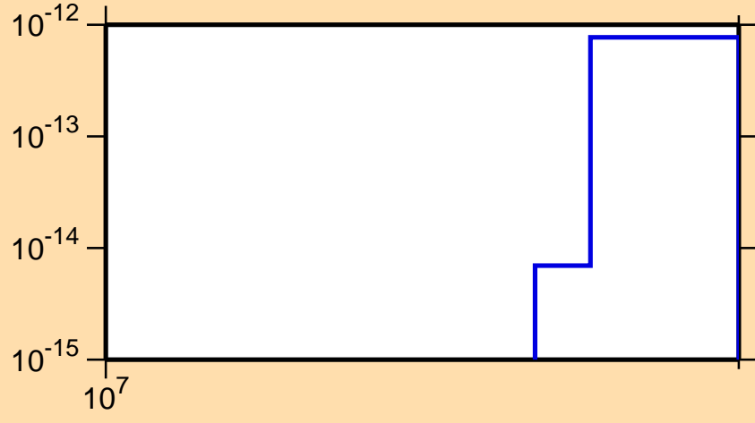
\sigma vs. E for ^{259}\text{Lw} (mt 34)
