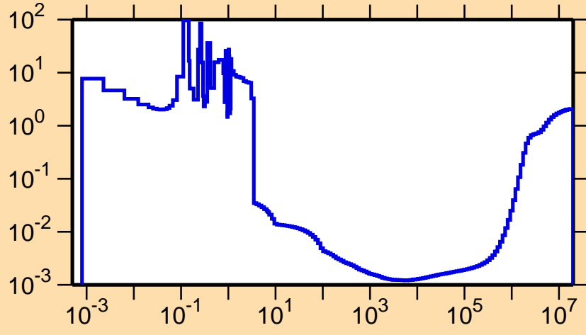
\sigma vs. E for ^{259}\text{Lw}(n,f)
