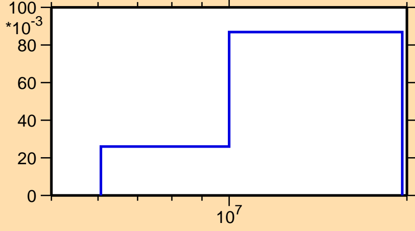
\sigma vs. E for ^{259}\text{Lw}(n,2n)
