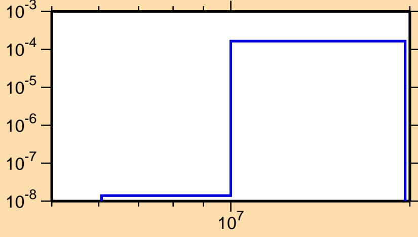
\sigma vs. E for ^{259}\text{Lw}(n,d)
