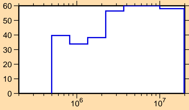
\Delta\sigma/\sigma vs. E for ^{259}\text{Lw}(n,n\text{cont.})
