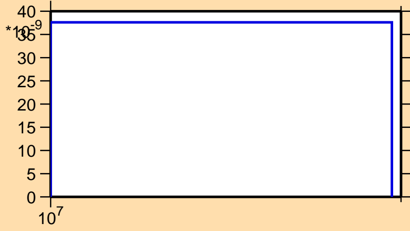
\sigma vs. E for ^{259}\text{Lw}(n,nd)
