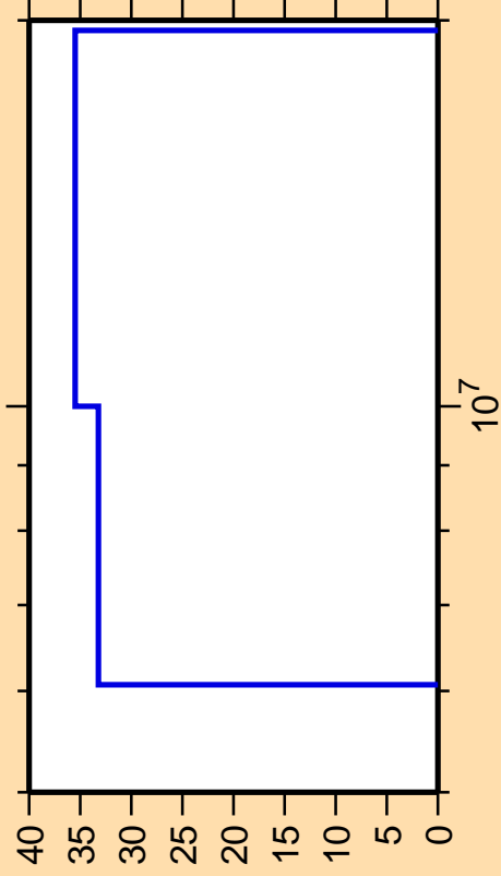
\Delta\sigma/\sigma vs. E for ^{259}\text{Lw}(n,d)
