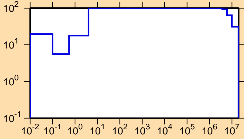
\Delta\sigma/\sigma vs. E for ^{259}\text{Lw}(n,f)
