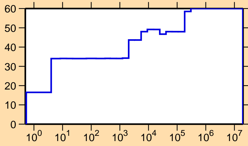
\Delta\sigma/\sigma vs. E for ^{259}\text{Lw}(n,\gamma)
