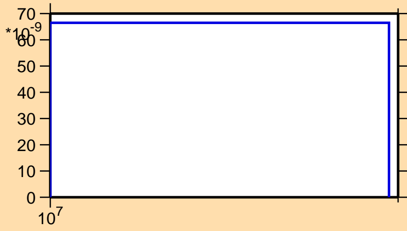
\sigma vs. E for ^{259}\text{Lw}(n,nt)
