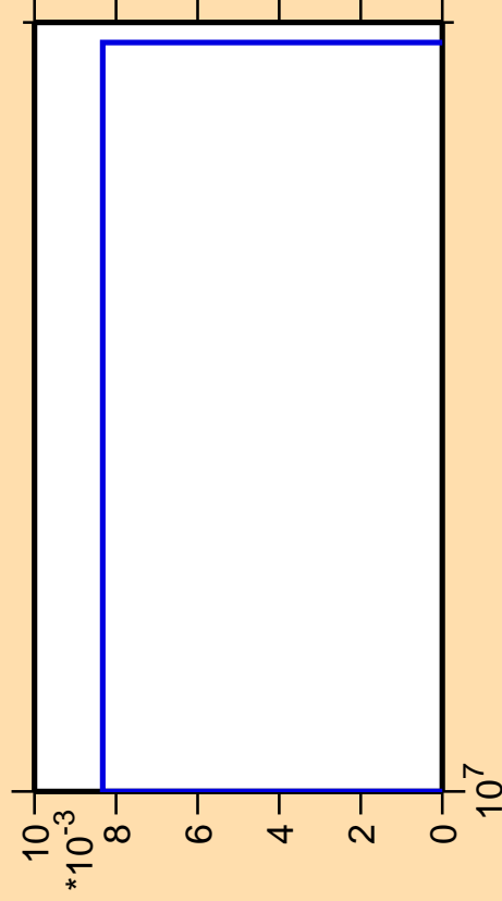
\Delta\sigma/\sigma vs. E for ^{259}\text{Lw} (mt 42)
