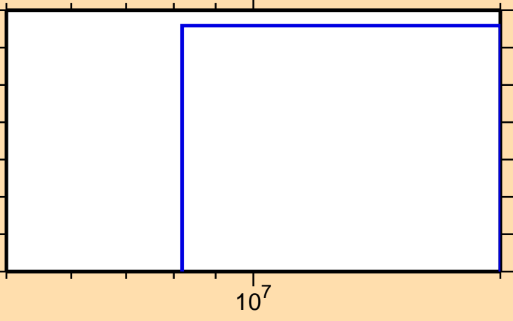
\sigma vs. E for ^{259}\text{Lw}(\text{mt } 34)
