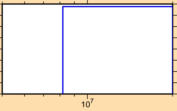
\sigma vs. E for ^{259}\text{Lw} (mt 42)
