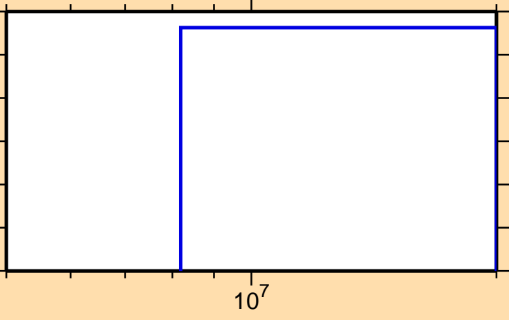
\sigma vs. E for ^{259}\text{Lw}(\text{mt 11})
