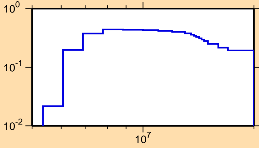
\sigma vs. E for ^{260}\text{Lw}(n,2n)
