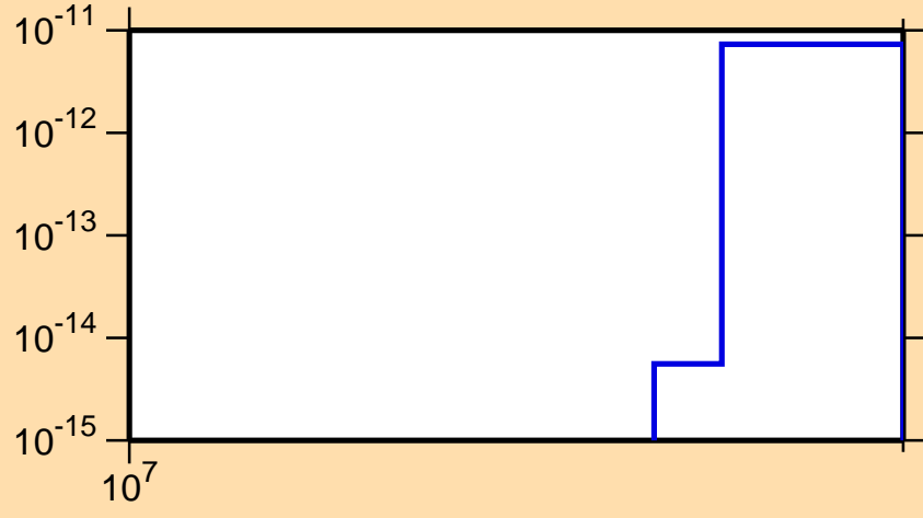
\sigma vs. E for ^{260}\text{Lw}(\text{mt 11})
