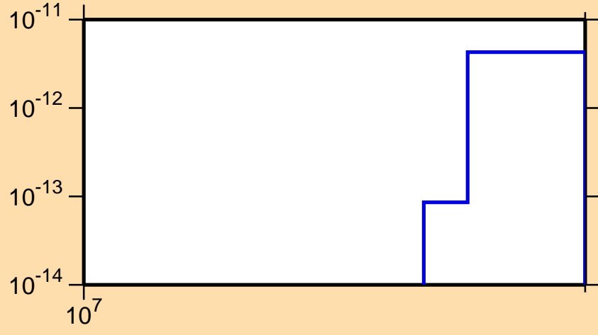
\sigma vs. E for ^{260}\text{Lw} (mt 34)
