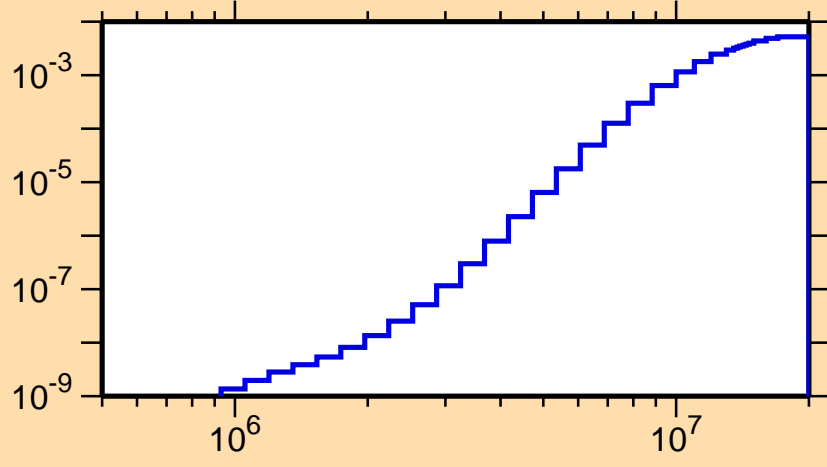
\sigma vs. E for ^{260}\text{Lw}(n,p)
