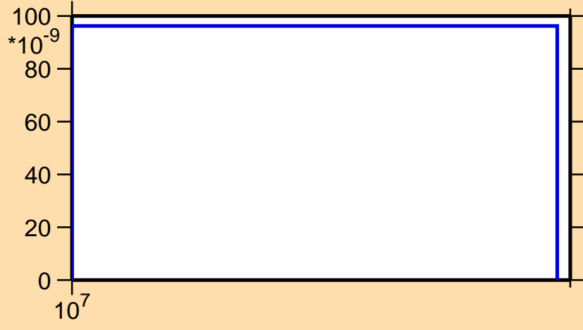
\sigma vs. E for ^{260}\text{Lw}(n,2np)
