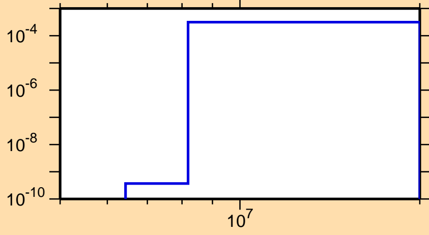
\sigma vs. E for ^{260}\text{Lw}(n,d)
