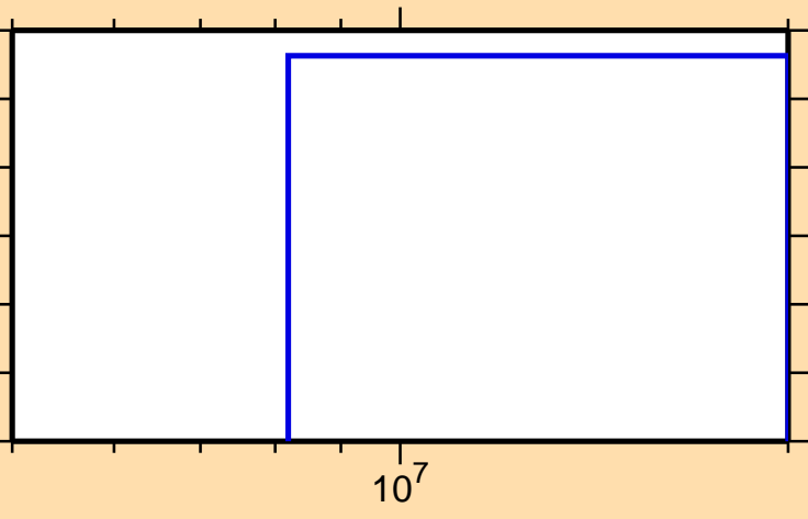
\sigma vs. E for ^{260}\text{Lw}(n,3n\alpha)
