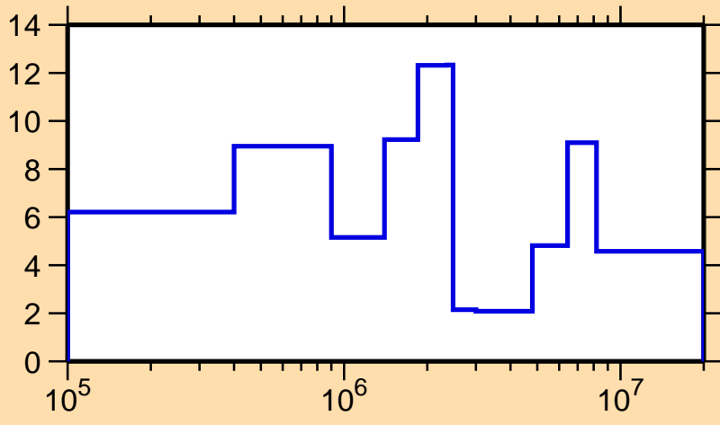
\Delta\sigma/\sigma vs. E for ^{260}\text{Lw}(n, tot.)
