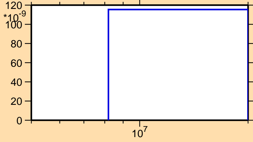
\sigma vs. E for ^{260}\text{Lw}(n,nt)
