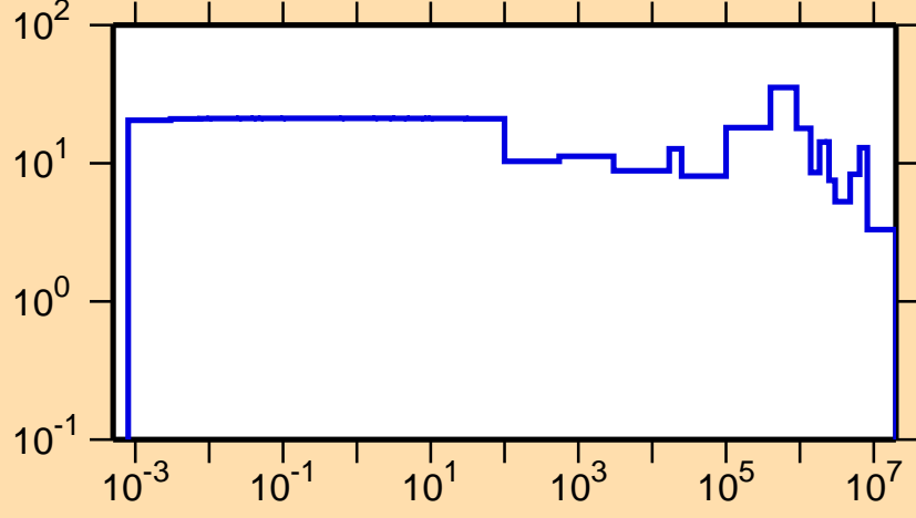
\Delta\sigma/\sigma vs. E for ^{260}\text{Lw}(n,el.)
