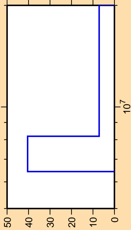
\Delta\sigma/\sigma vs. E for ^{260}\text{Lw}(n,d)
