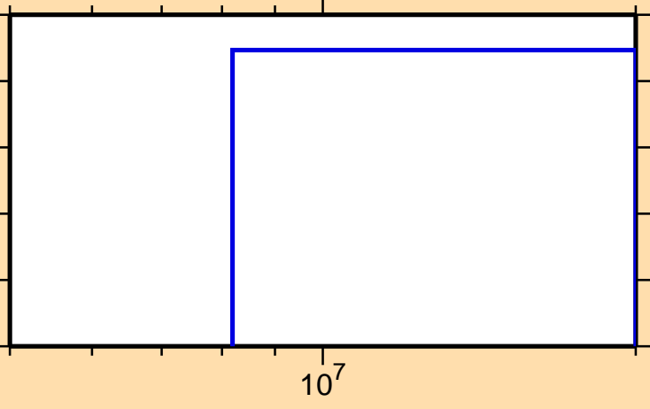
\sigma vs. E for ^{260}\text{Lw}(n,nd)
