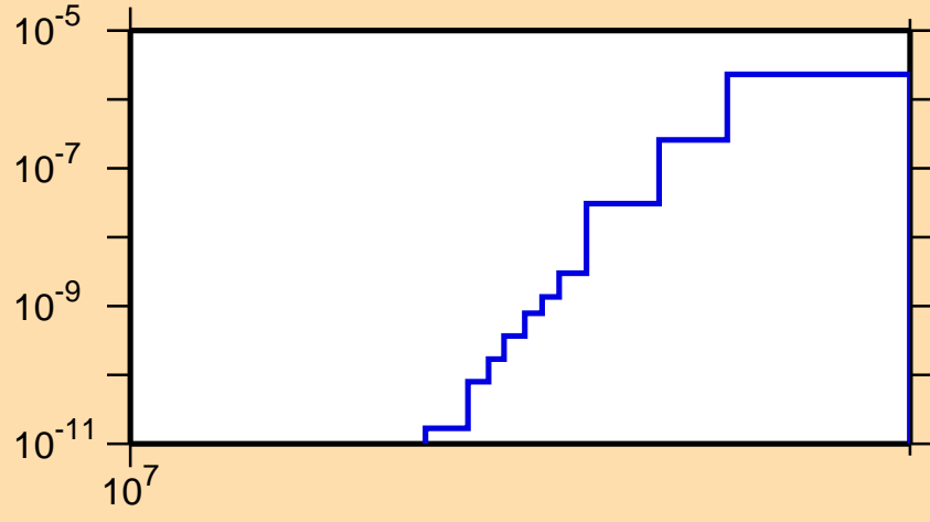
\sigma vs. E for ^{261}\text{Lw}(n,nd)
