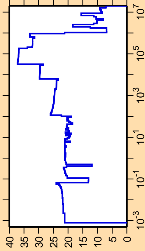
\Delta\sigma/\sigma vs. E for ^{261}\text{Lw}(n,\text{el.})
