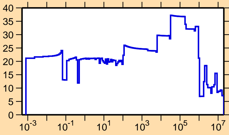
\Delta\sigma/\sigma vs. E for ^{261}\text{Lw}(n,el.)
