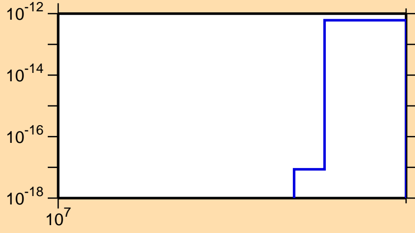
\sigma vs. E for ^{261}\text{Lw} (mt 42)
