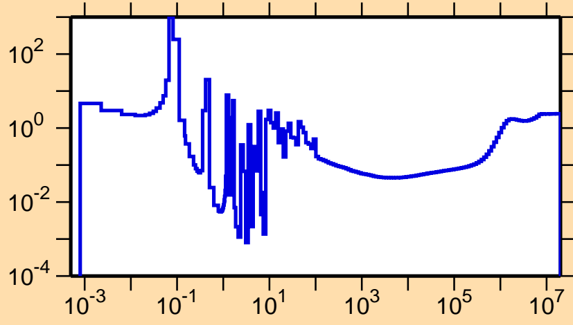
\sigma vs. E for ^{261}\text{Lw}(n,f)
