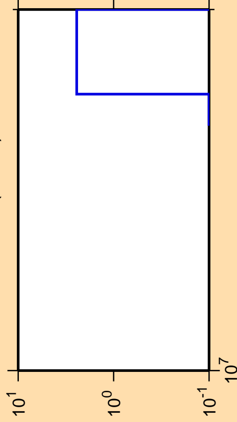
\Delta\sigma/\sigma vs. E for ^{261}\text{Lw}(\text{mt } 11)
