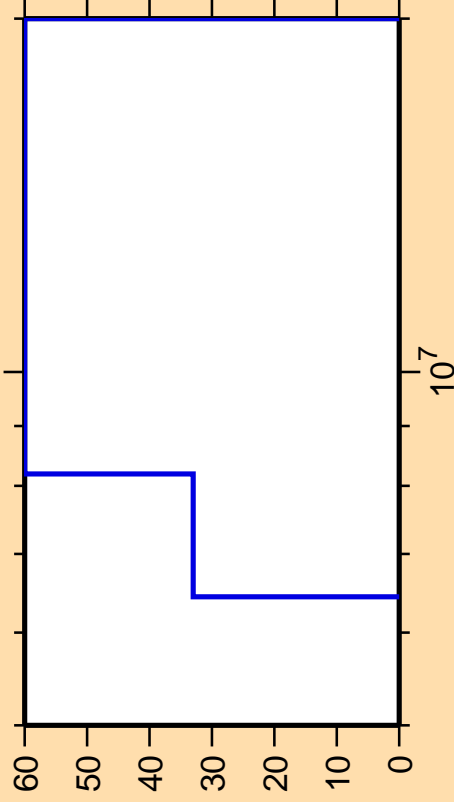
\Delta\sigma/\sigma vs. E for ^{261}\text{Lw}(\text{mt117})
