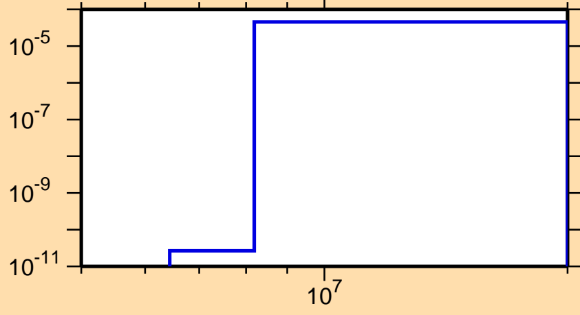
\sigma vs. E for ^{261}\text{Lw}(n,np)
