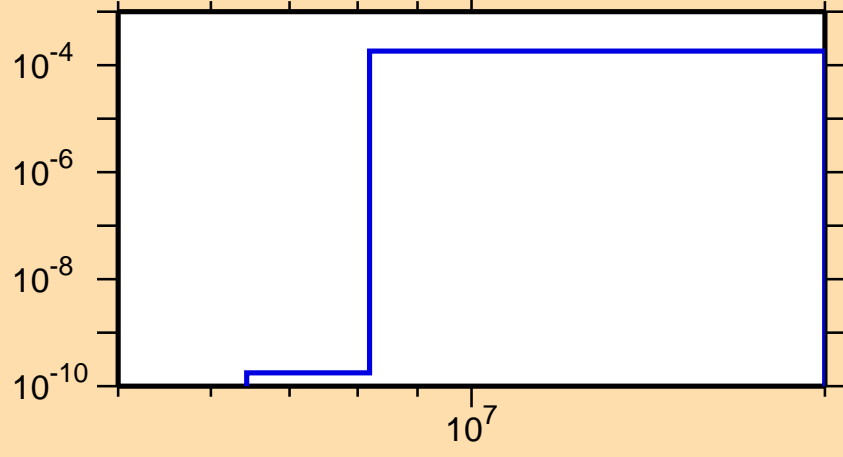
\sigma vs. E for ^{261}\text{Lw}(\text{mt117})
