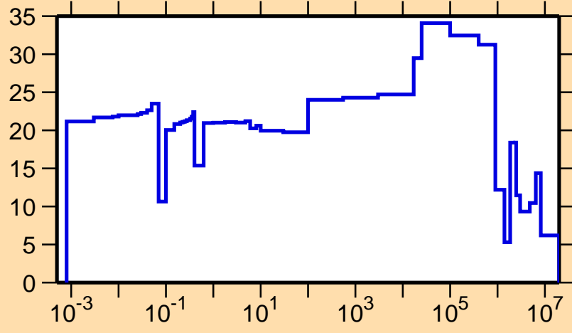
\Delta\sigma/\sigma vs. E for ^{261}\text{Lw}(n,el.)
