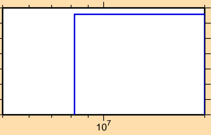
\sigma vs. E for ^{261}\text{Lw}(n,nd)
