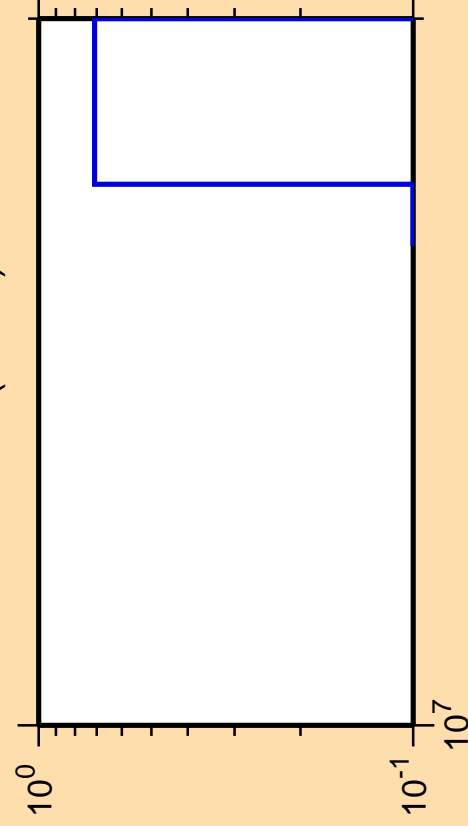
\Delta\sigma/\sigma vs. E for ^{262}\text{Lw} (mt 42)
