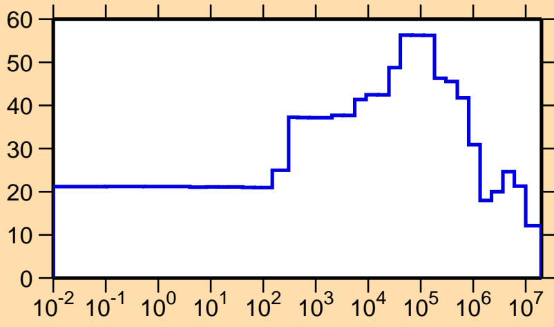
\Delta\sigma/\sigma vs. E for ^{262}\text{Lw}(n,el.)
