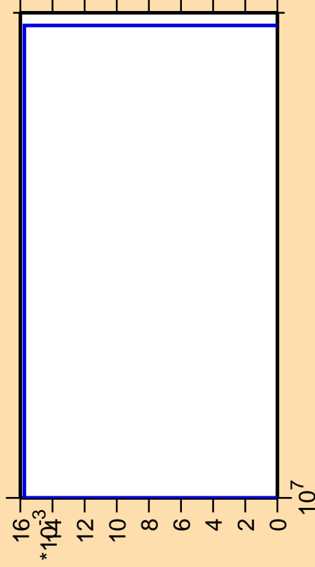
\Delta\sigma/\sigma vs. E for ^{262}\text{Lw} (mt 34)
