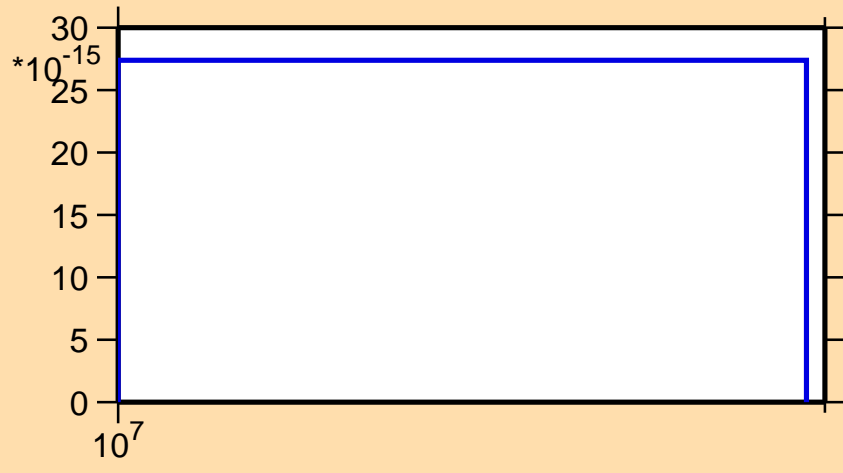
\sigma vs. E for ^{262}\text{Lw}(\text{mt 11})
