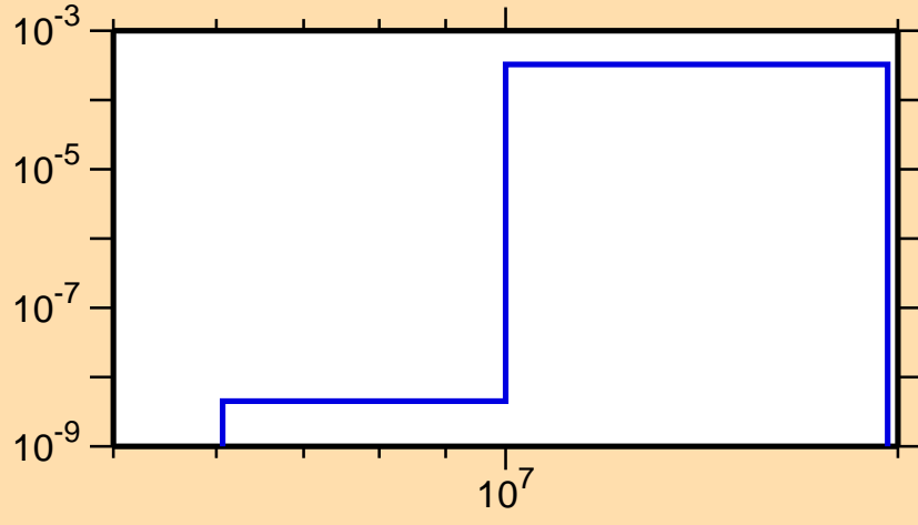
\sigma vs. E for ^{262}\text{Lw}(n,d)
