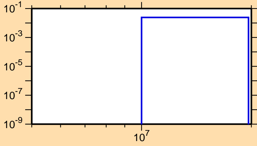
\sigma vs. E for ^{262}\text{Lw}(n,3n\alpha)
