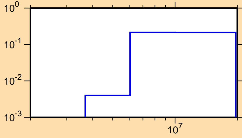
\sigma vs. E for ^{262}\text{Lw}(n,2n)
