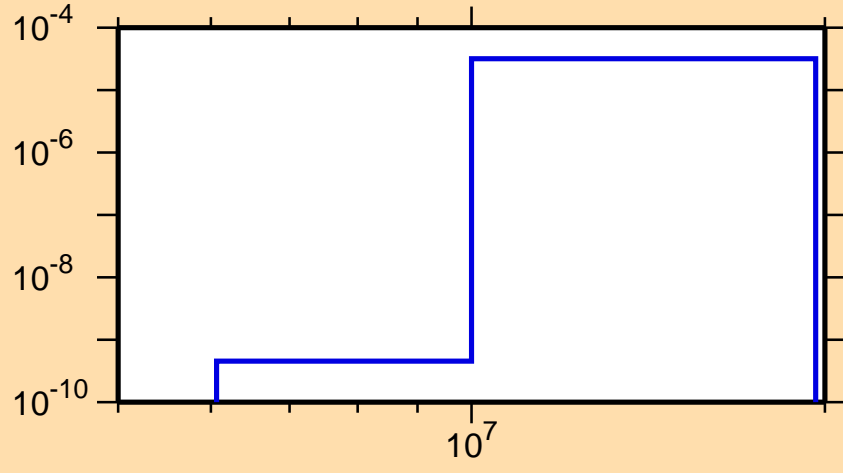
\sigma vs. E for ^{262}\text{Lw}(\text{mt117})
