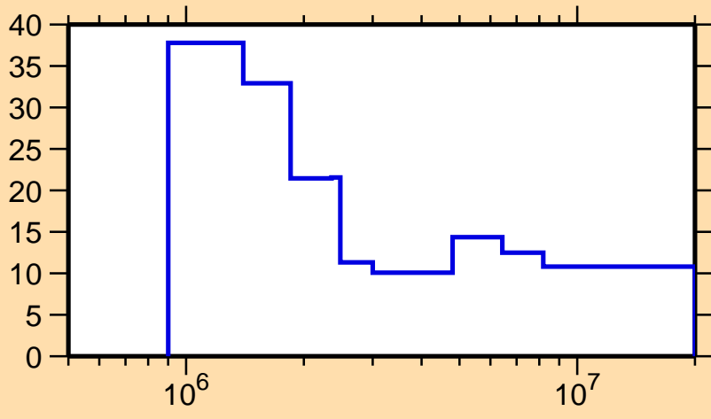
\Delta\sigma/\sigma vs. E for ^{262}\text{Lw}(n,\text{nonel.})
