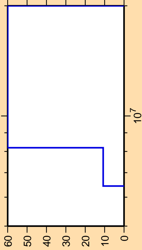
\Delta\sigma/\sigma vs. E for ^{262}\text{Lw}(n,np)
