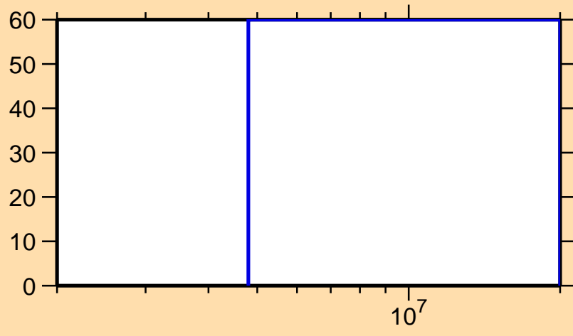
\Delta\sigma/\sigma vs. E for ^{262}\text{Lw}(n,2n)
