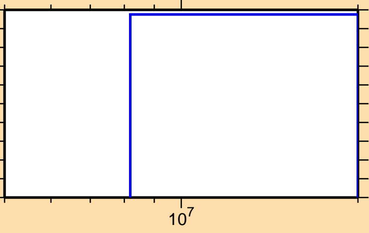
\sigma vs. E for ^{262}\text{Lw}(n,3n\alpha)
