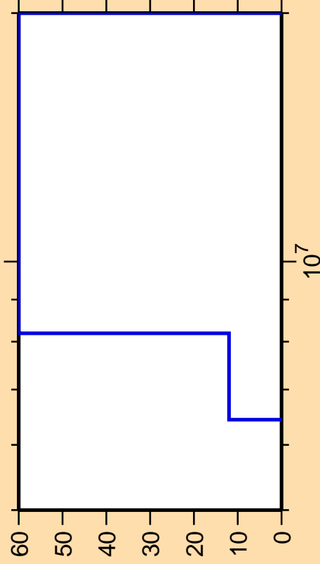
\Delta\sigma/\sigma vs. E for ^{262}\text{Lw}(n,t)
