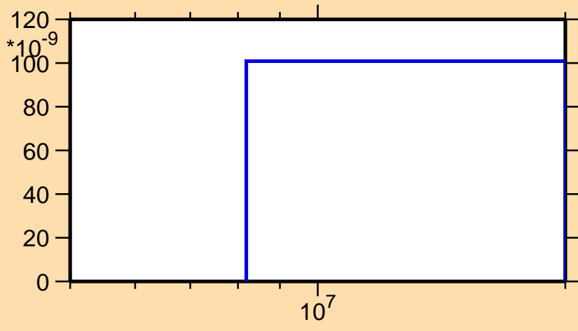
\sigma vs. E for ^{262}\text{Lw}(n,nt)
