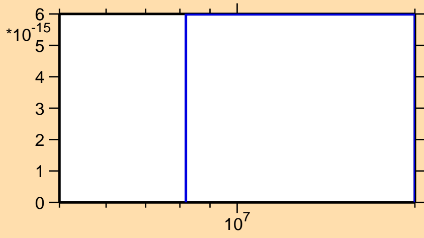
\sigma vs. E for ^{262}\text{Lw} (mt 42)
