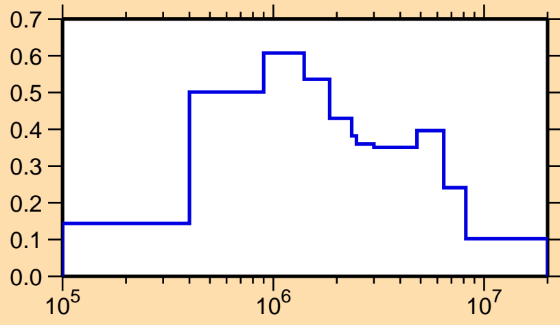
\sigma vs. E for ^{262}\text{Lw}(n,n\text{cont.})
