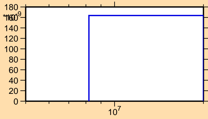
\sigma vs. E for ^{262}\text{Lw}(n,nd)
