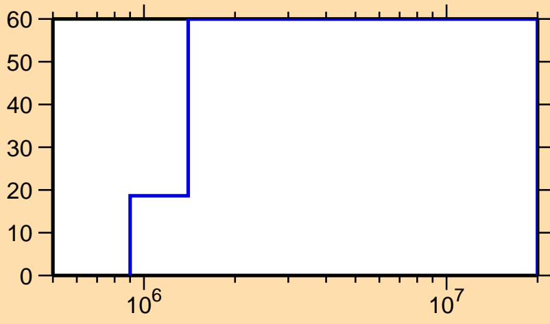
\Delta\sigma/\sigma vs. E for ^{262}\text{Lw}(n,p)
