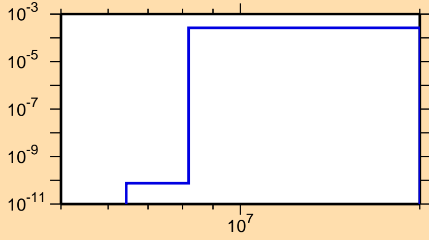
\sigma vs. E for ^{262}\text{Lw}(n,d)
