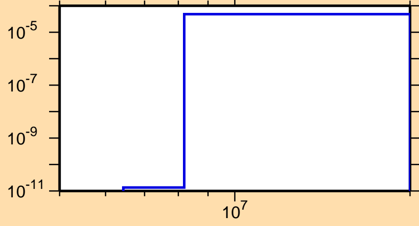
\sigma vs. E for ^{262}\text{Lw}(n,t)
