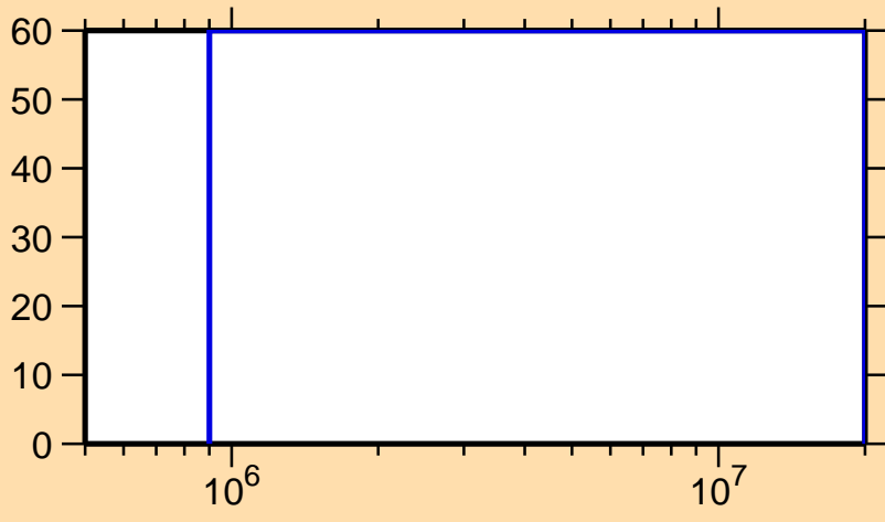
\Delta\sigma/\sigma vs. E for ^{262}\text{Lw}(n,\gamma)
