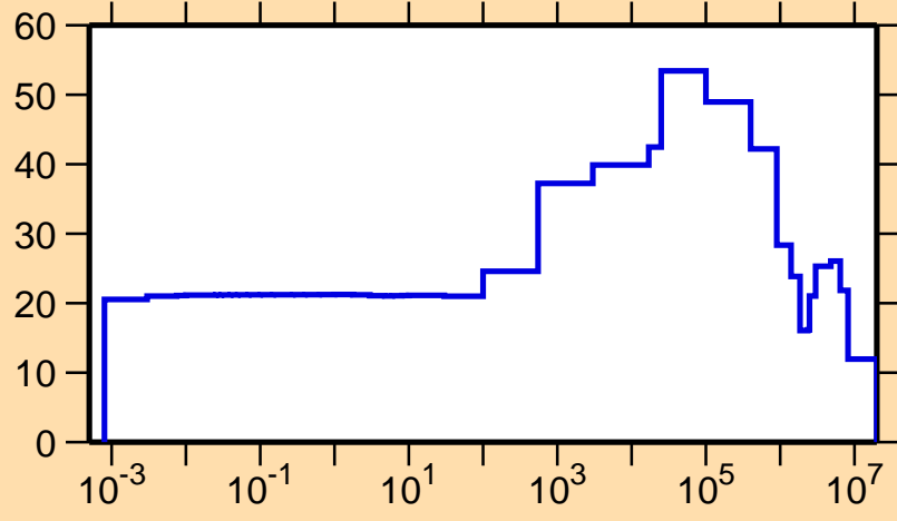
\Delta\sigma/\sigma vs. E for ^{262}\text{Lw}(n,el.)
