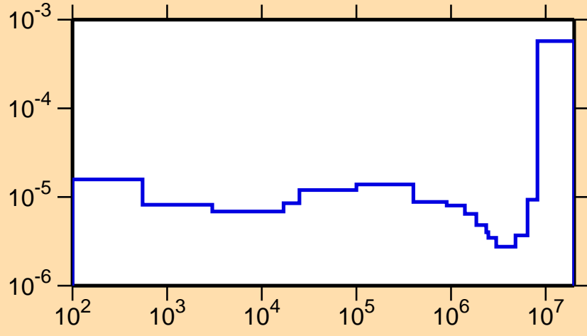
\sigma vs. E for ^{262}\text{Lw}(n, \alpha)
