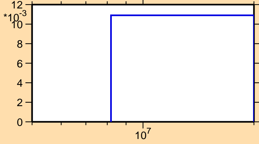
\sigma vs. E for ^{262}\text{Lw}(n,3n)
