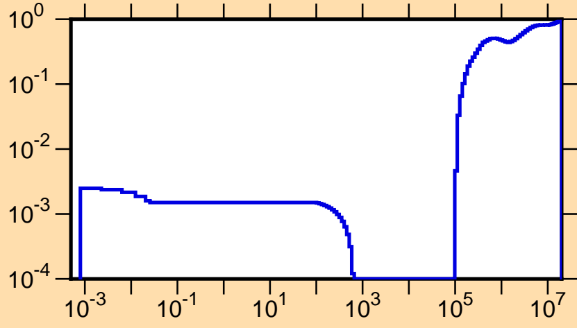
\mu vs. E for ^{263}\text{Lw}(\text{mt251})
