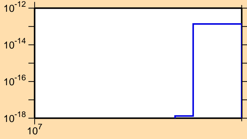
\sigma vs. E for ^{263}\text{Lw} (mt 42)
