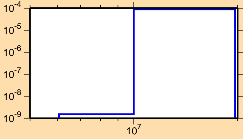
\sigma vs. E for ^{263}\text{Lw}(\text{mt117})
