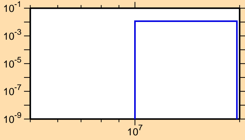
\sigma vs. E for ^{263}\text{Lw}(n,3n\alpha)
