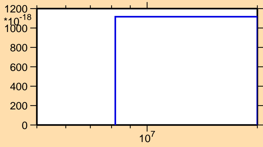
\sigma vs. E for ^{263}\text{Lw}(\text{mt } 42)
