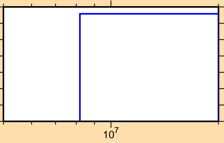
\sigma vs. E for ^{263}\text{Lw}(n,\text{He3})
