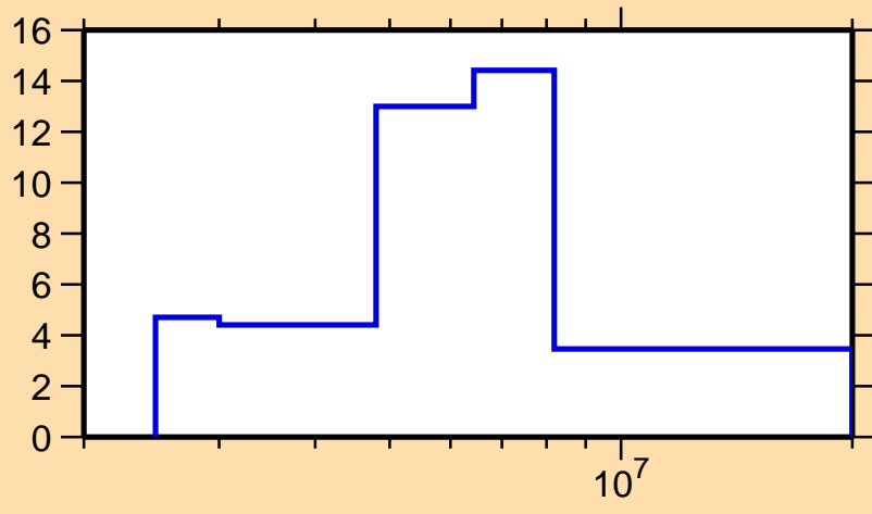
\Delta\sigma/\sigma vs. E for ^{263}\text{Lw}(n,el.)
