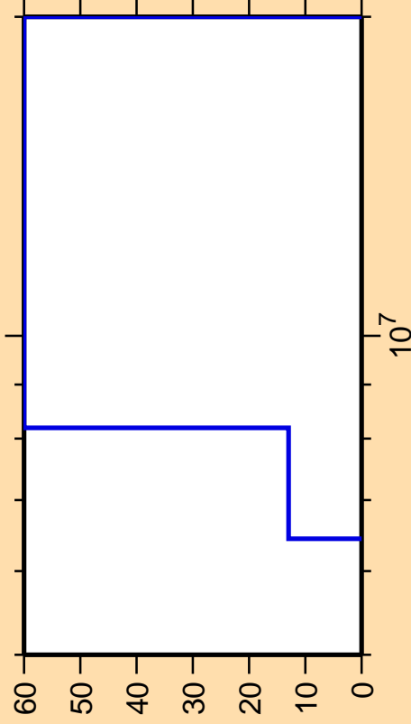
\Delta\sigma/\sigma vs. E for ^{263}\text{Lw}(\text{mt117})
