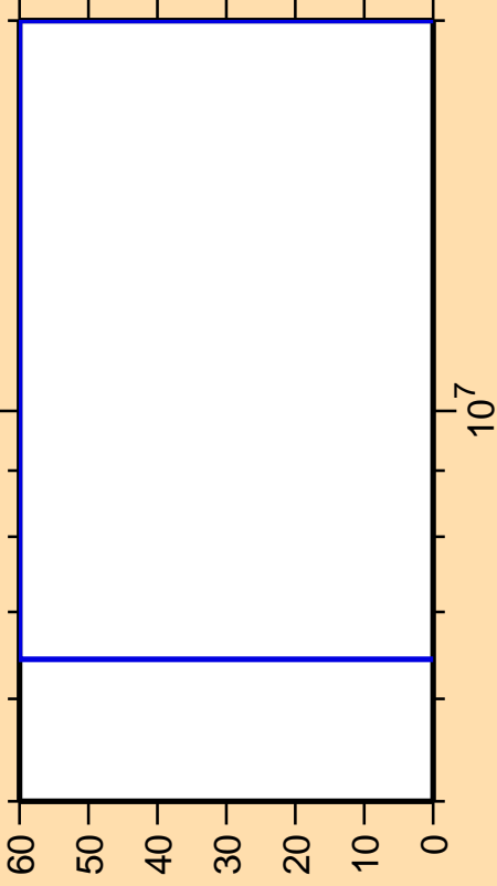
\Delta\sigma/\sigma vs. E for ^{263}\text{Lw}(n, n_{\text{cont}})
