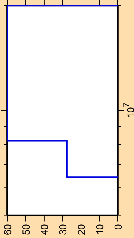
\Delta\sigma/\sigma vs. E for ^{263}\text{Lw}(n,d)
