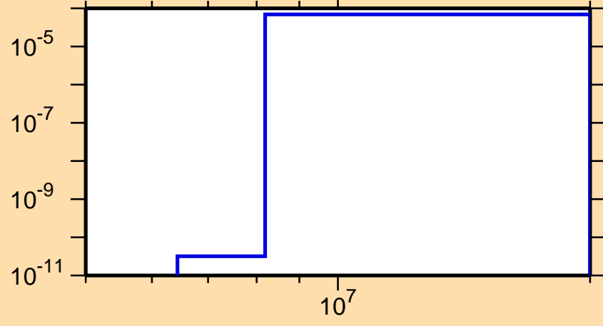
\sigma vs. E for ^{263}\text{Lw}(\text{mt117})
