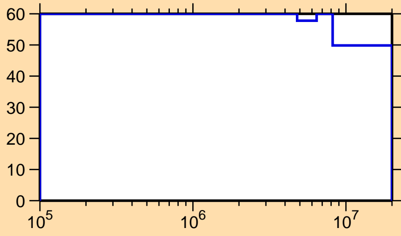
\Delta\sigma/\sigma vs. E for ^{263}\text{Lw}(n,n_1)
