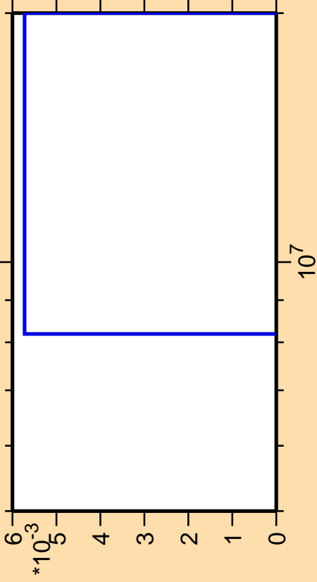
\Delta\sigma/\sigma vs. E for ^{263}\text{Lw}(\text{mt } 42)
