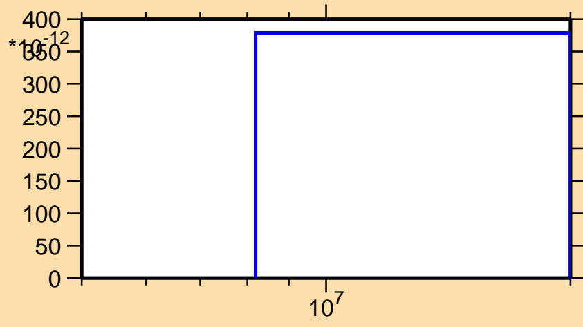
\sigma vs. E for ^{263}\text{Lw}(n,2np)
