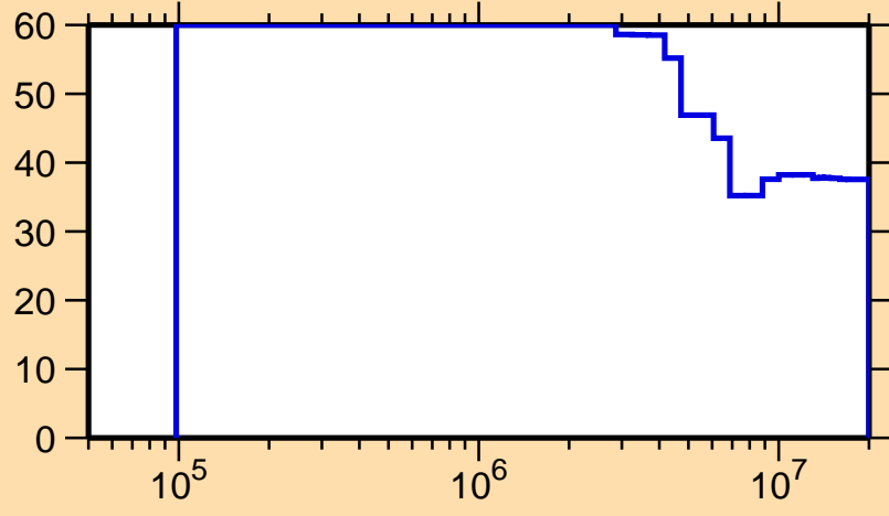
\Delta\sigma/\sigma vs. E for ^{264}\text{Lw}(n, n_{\text{cont}})
