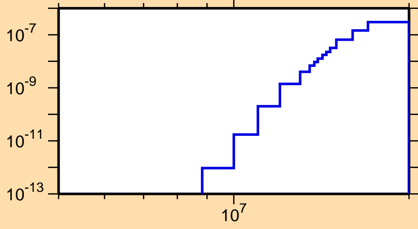
\sigma vs. E for ^{264}\text{Lw}(\text{mt117})
