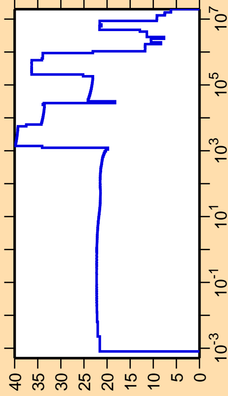
\Delta\sigma/\sigma vs. E for ^{264}\text{Lw}(n,\text{el.})
