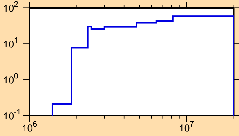
\Delta\sigma/\sigma vs. E for ^{264}\text{Lw}(n,p)
