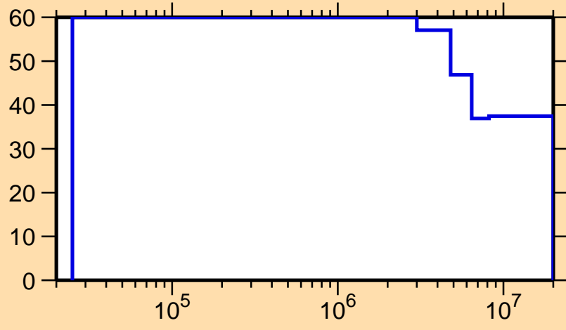
\Delta\sigma/\sigma vs. E for ^{264}\text{Lw}(n, n\text{cont.})
