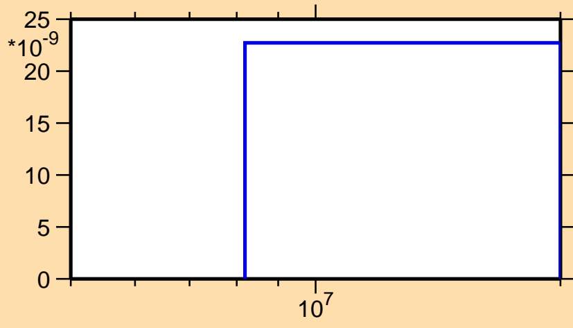
\sigma vs. E for ^{264}\text{Lw}(\text{mt117})
