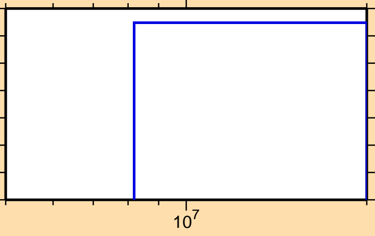
\sigma vs. E for ^{264}\text{Lw}(n,\text{He3})
