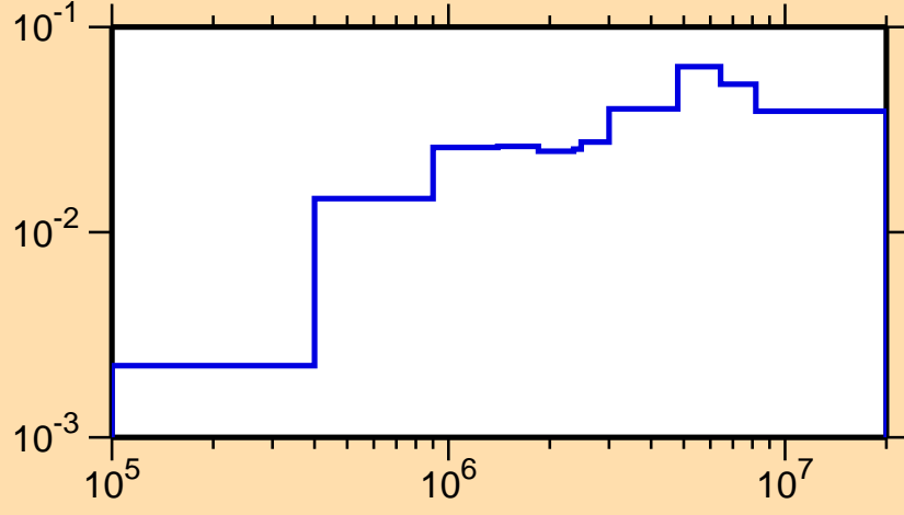
\sigma vs. E for ^{264}\text{Lw}(n,n\alpha)
