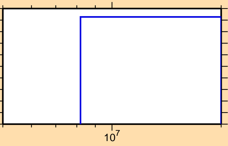
\sigma vs. E for ^{264}\text{Lw}(n,nd)
