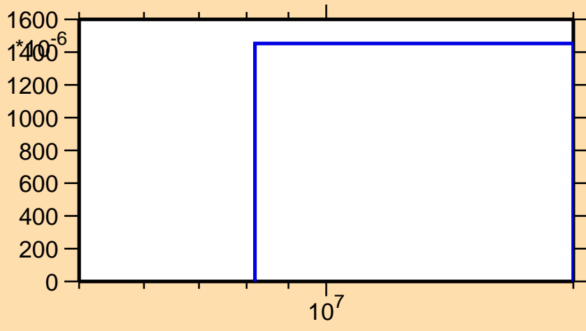
\sigma vs. E for ^{265}\text{Lw}(n,3n)
