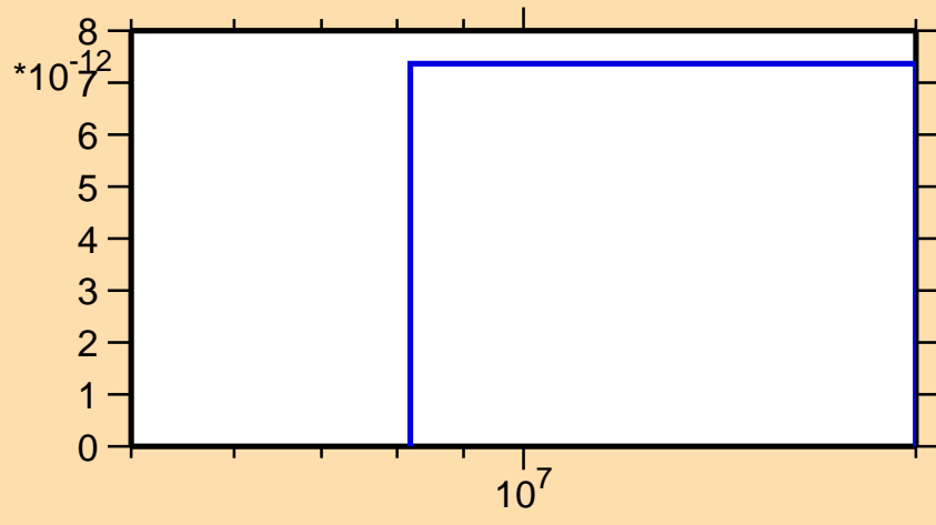
\sigma vs. E for ^{265}\text{Lw}(n,2np)
