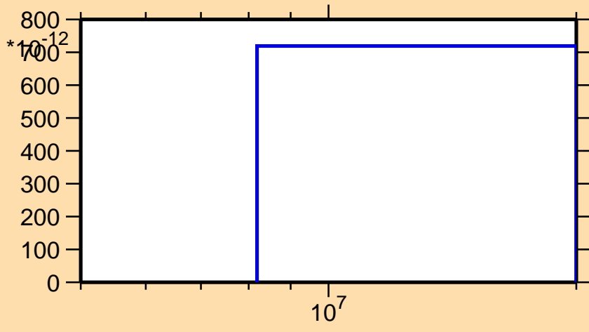
\sigma vs. E for ^{265}\text{Lw}(n,nd)
