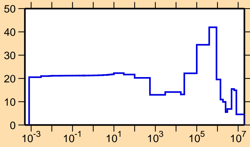
\Delta\sigma/\sigma vs. E for ^{265}\text{Lw}(n,el.)
