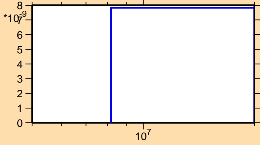
\sigma vs. E for ^{265}\text{Lw}(n,nt)
