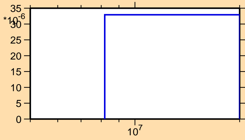
\sigma vs. E for ^{265}\text{Lw}(n,t)
