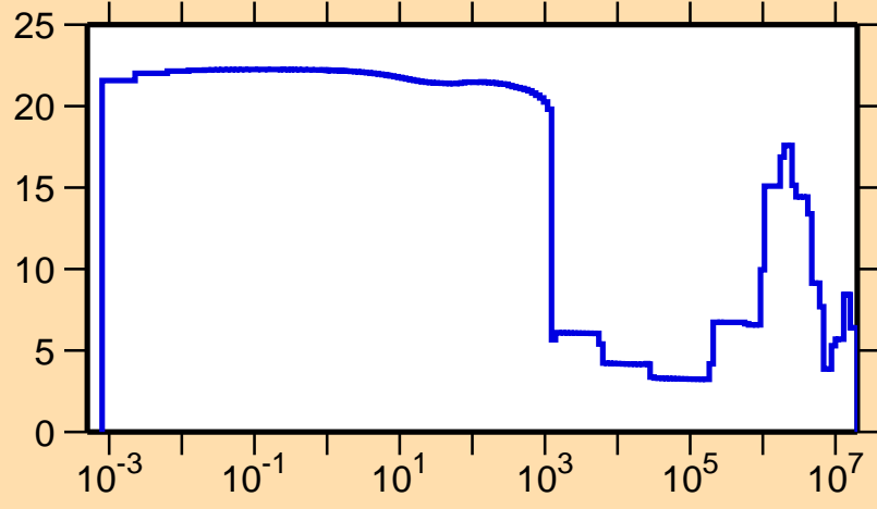
\Delta\sigma/\sigma vs. E for ^{266}\text{Lw}(n,el.)
