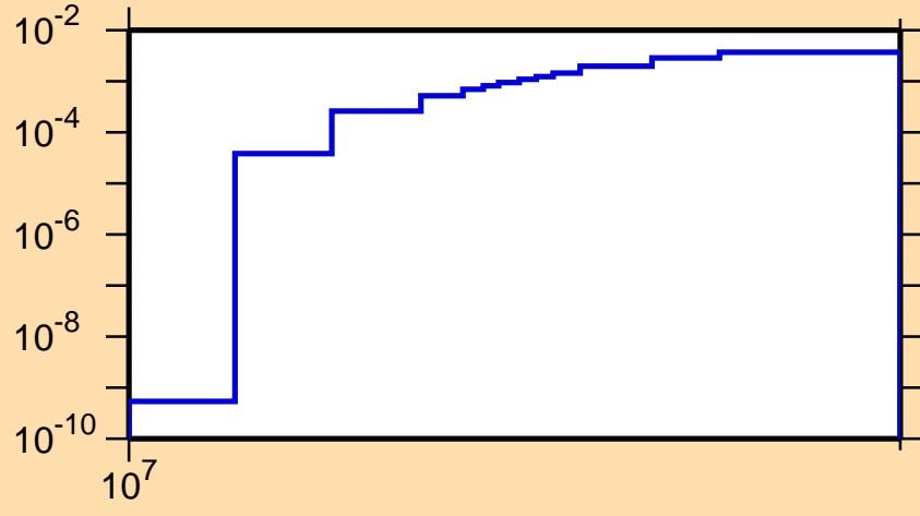
\sigma vs. E for ^{266}\text{Lw}(n,3n)
