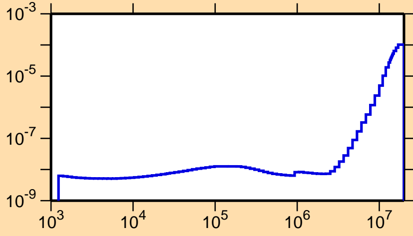
\sigma vs. E for ^{266}\text{Lw}(n,\alpha)
