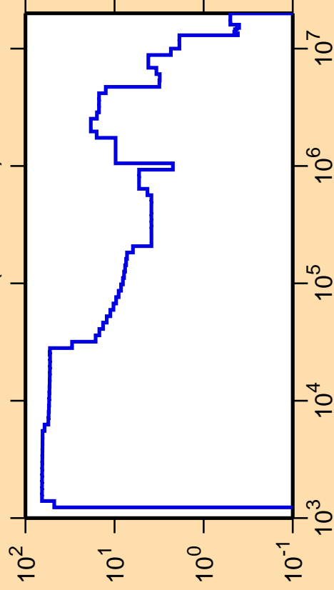
\Delta\sigma/\sigma vs. E for ^{266}\text{Lw}(n,\text{nonel.})
