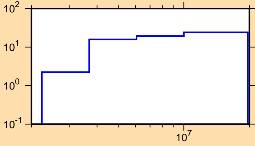
\Delta\sigma/\sigma vs. E for ^{266}\text{Lw}(n,p)
