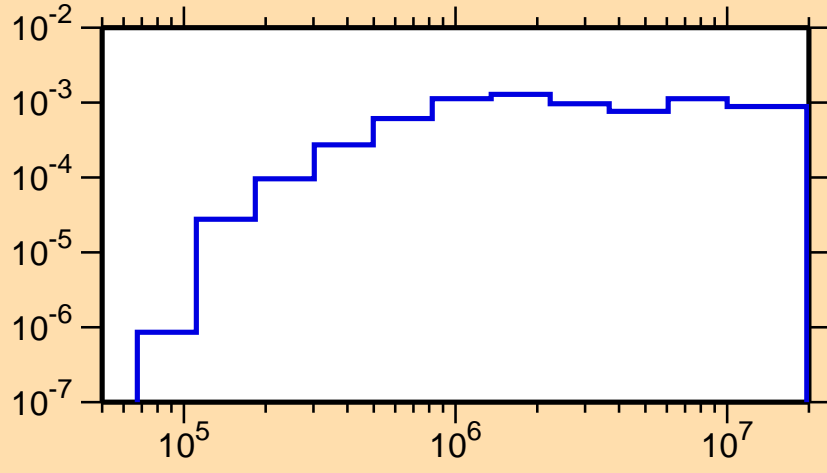
\sigma vs. E for ^{266}\text{Lw}(n,n\alpha)
