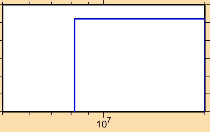
\sigma vs. E for ^{266}\text{Lw}(n,nd)
