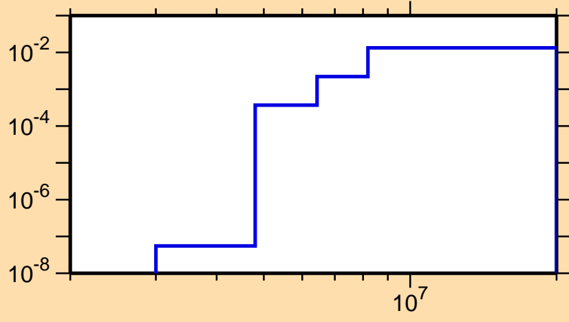
\sigma vs. E for ^{266}\text{Lw}(n,2n)
