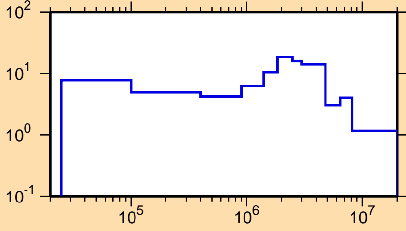
\Delta\sigma/\sigma vs. E for ^{266}\text{Lu}(n,\text{nonel.})
