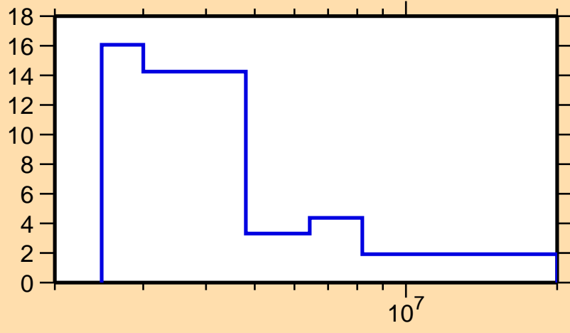
\Delta\sigma/\sigma vs. E for ^{266}\text{Lw}(n,f)
