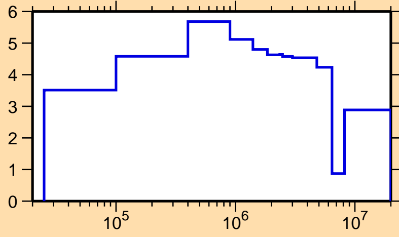
\Delta\sigma/\sigma vs. E for ^{266}\text{Lw}(n,\text{tot.})
