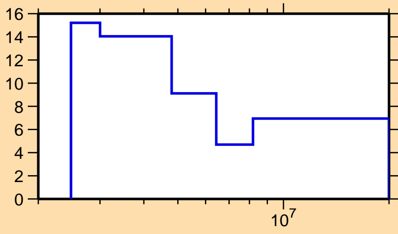
\Delta\sigma/\sigma vs. E for ^{266}\text{Lw}(n,el.)
