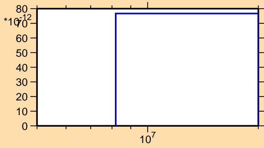
\sigma vs. E for ^{266}\text{Lw}(n,2np)
