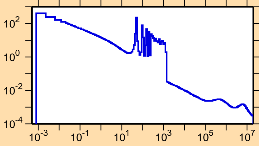
\sigma vs. E for ^{154}\text{Lu}(n,\gamma)
