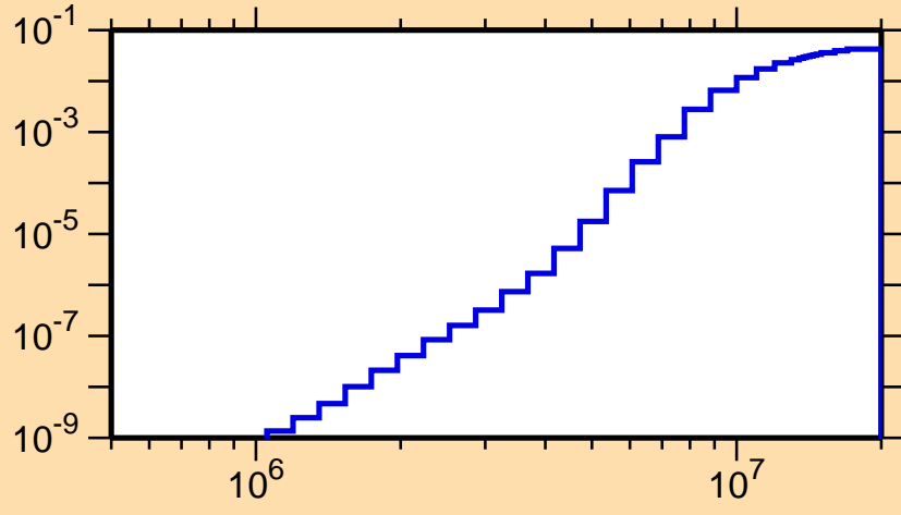
\sigma vs. E for ^{154}\text{Lu}(n,d)
