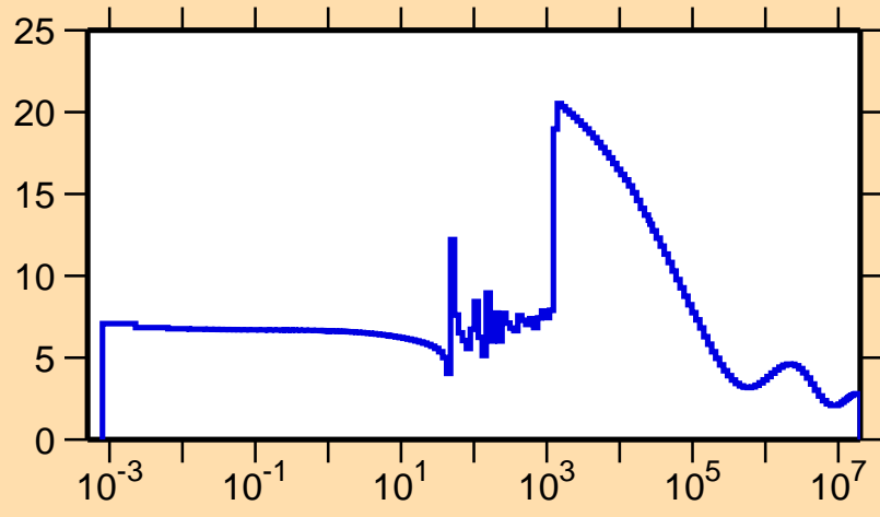
\sigma vs. E for ^{154}\text{Lu}(n,\text{el.})
