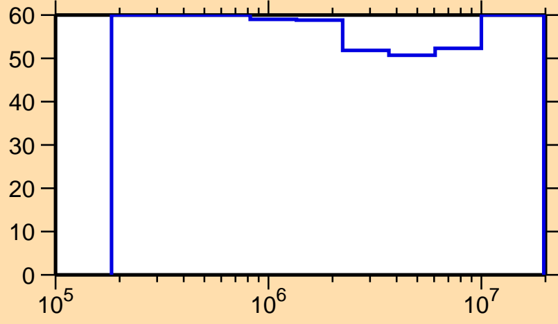
\Delta\sigma/\sigma vs. E for ^{154}\text{Lu}(n,n_1)
