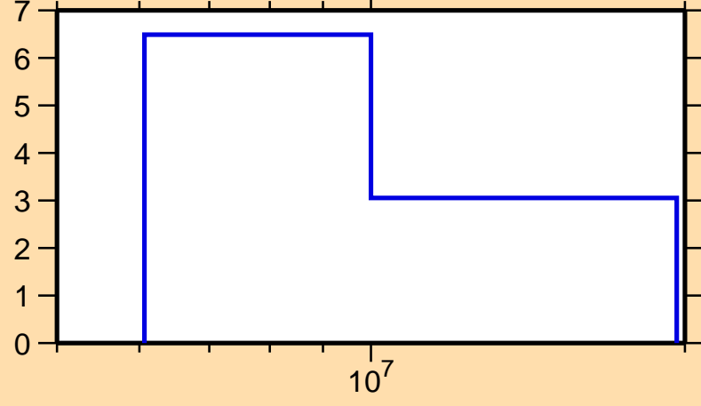
\Delta\sigma/\sigma vs. E for ^{154}\text{Lu}(n,\text{tot.})
