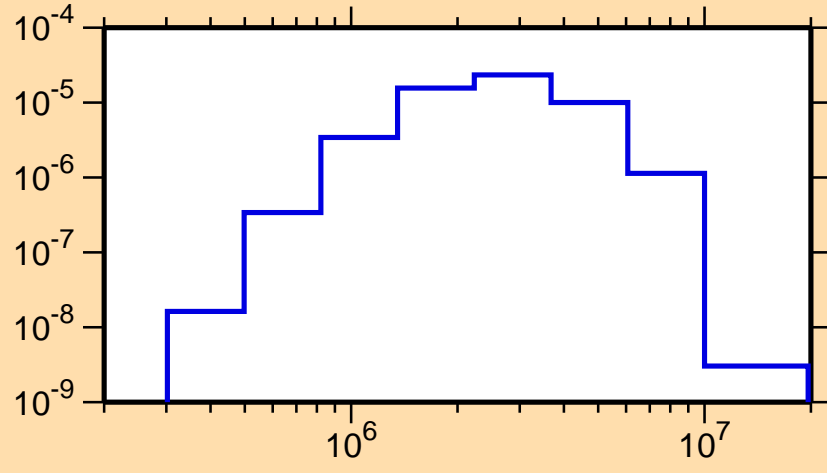
\sigma vs. E for ^{154}\text{Lu}(n,n_1)
