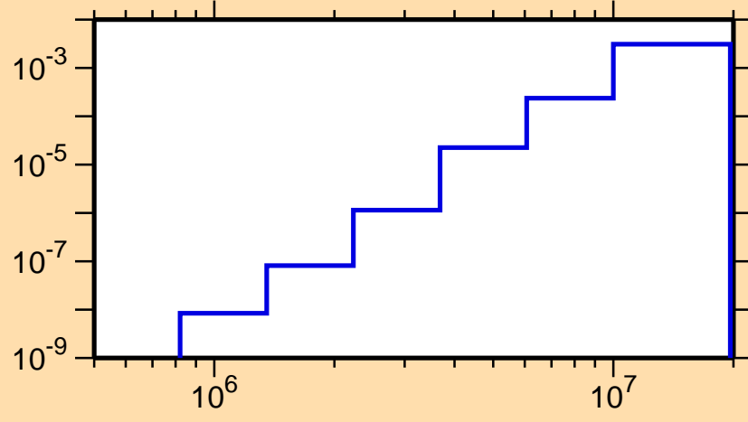
\sigma vs. E for ^{154}\text{Lu}(n,n\alpha)
