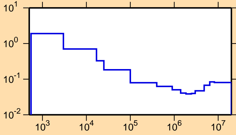
\sigma vs. E for ^{154}\text{Lu}(n,\alpha)
