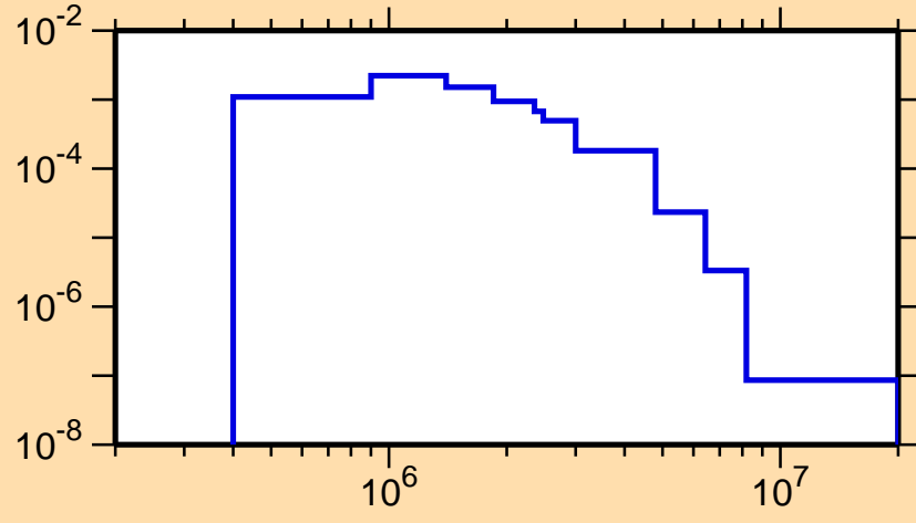
\sigma vs. E for ^{154}\text{Lu}(n,n_3)
