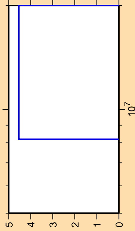
\Delta\sigma/\sigma vs. E for ^{154}\text{Lu}(n,nt)
