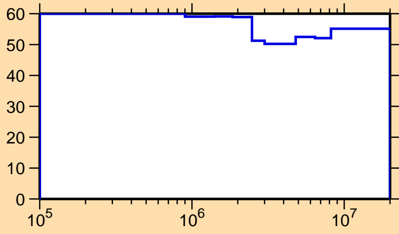
\Delta\sigma/\sigma vs. E for ^{154}\text{Lu}(n,n_1)
