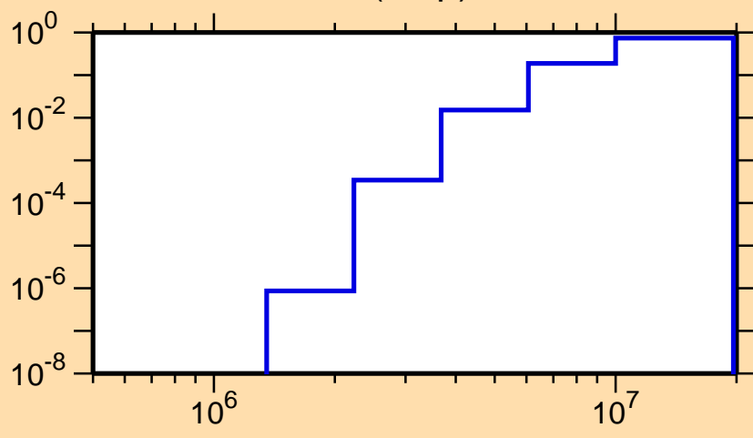
\sigma vs. E for ^{154}\text{Lu}(n,np)
