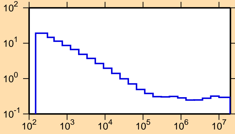
\sigma vs. E for ^{154}\text{Lu}(n,p\alpha)
