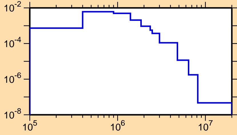
\sigma vs. E for ^{154}\text{Lu}(n,n_2)
