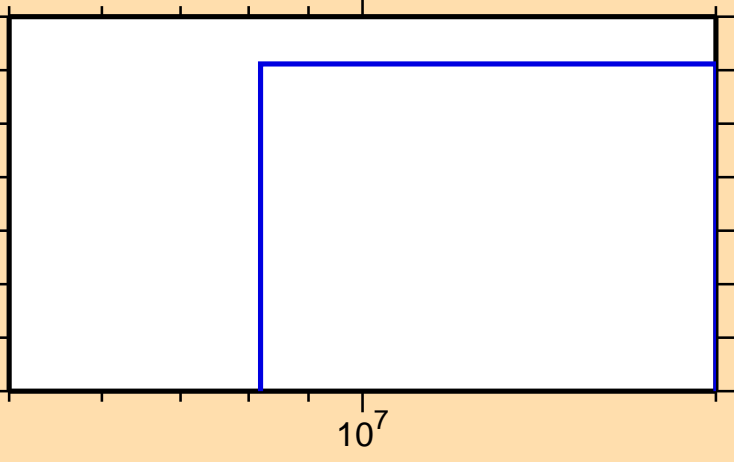
\sigma vs. E for ^{154}\text{Lu}(n,\text{pt})
