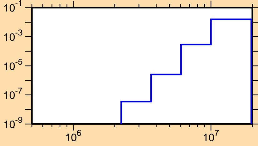
\sigma vs. E for ^{157}\text{Lu}(n,d)
