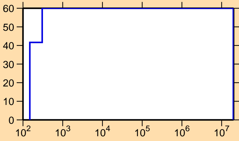
\Delta\sigma/\sigma vs. E for ^{157}\text{Lu}(n,p)
