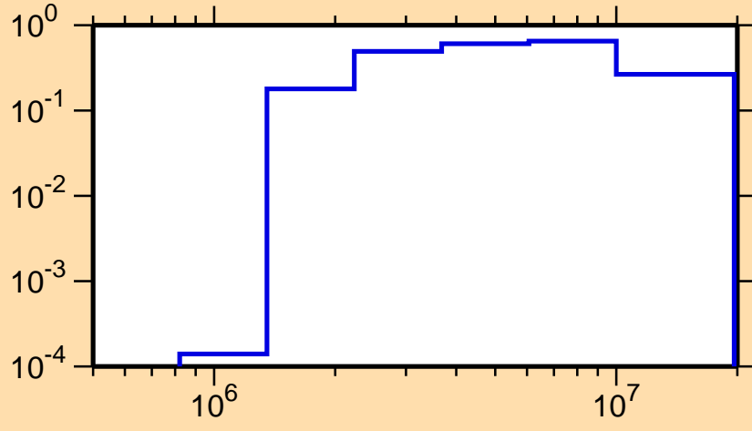
\sigma vs. E for ^{157}\text{Lu}(n,n\text{cont.})
