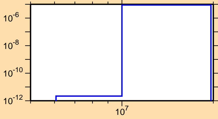
\sigma vs. E for ^{157}\text{Lu}(n,p,d)
