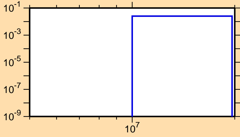
\sigma vs. E for ^{157}\text{Lu}(n,2n\alpha)
