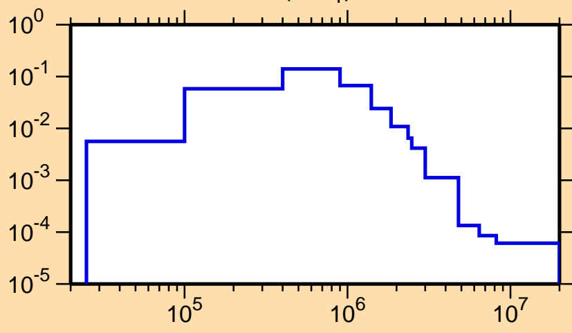
\sigma vs. E for ^{157}\text{Lu}(n,n_1)
