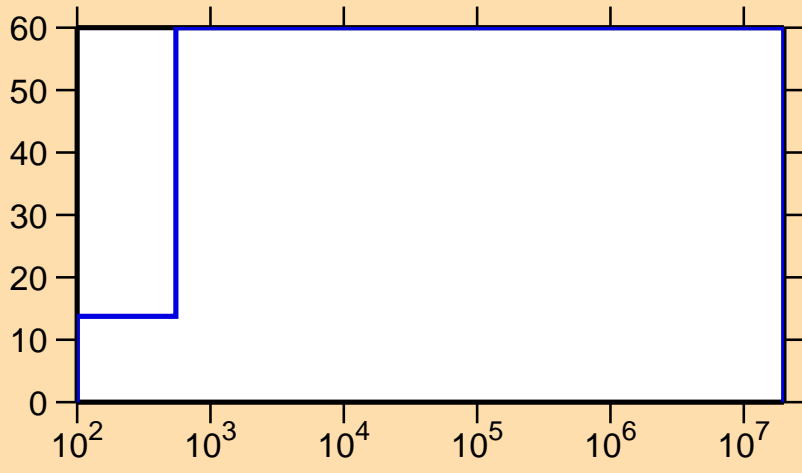
\Delta\sigma/\sigma vs. E for ^{157}\text{Lu}(n,\gamma)
