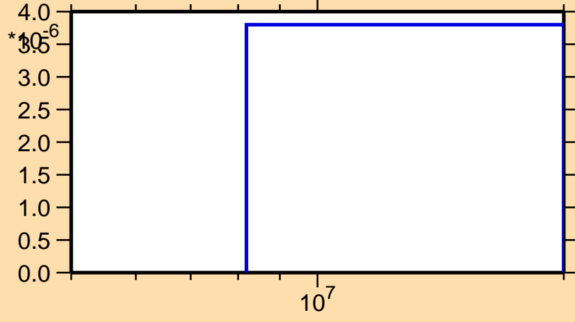
\sigma vs. E for ^{157}\text{Lu}(n,pd)
