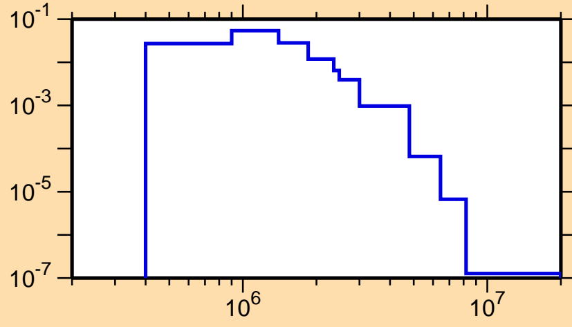
\sigma vs. E for ^{157}\text{Lu}(n,n_2)
