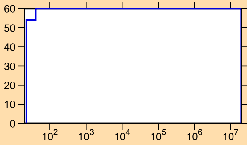
\Delta\sigma/\sigma vs. E for ^{158}\text{Lu}(n,\gamma)
