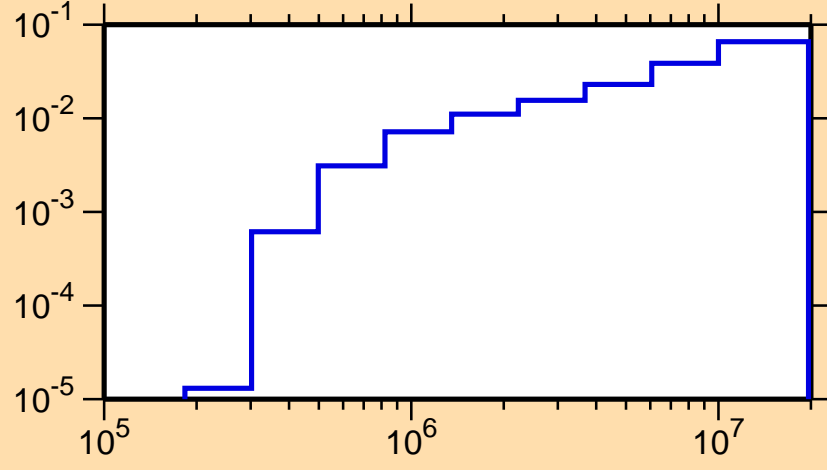
\sigma vs. E for ^{158}\text{Lu}(n,n\alpha)
