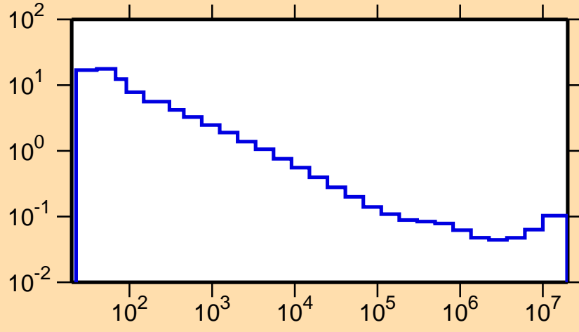
\sigma vs. E for ^{158}\text{Lu}(n,\alpha)
