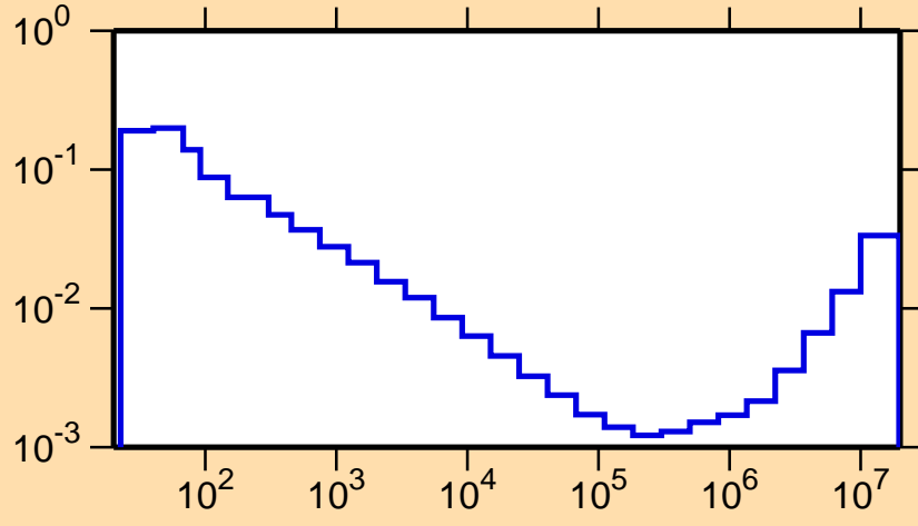
\sigma vs. E for ^{158}\text{Lu}(n,p\alpha)
