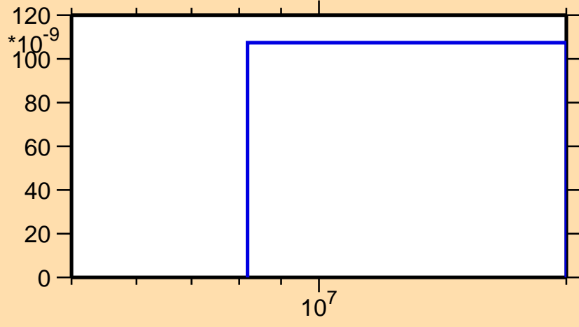
\sigma vs. E for ^{158}\text{Lu}(n,\text{pt})
