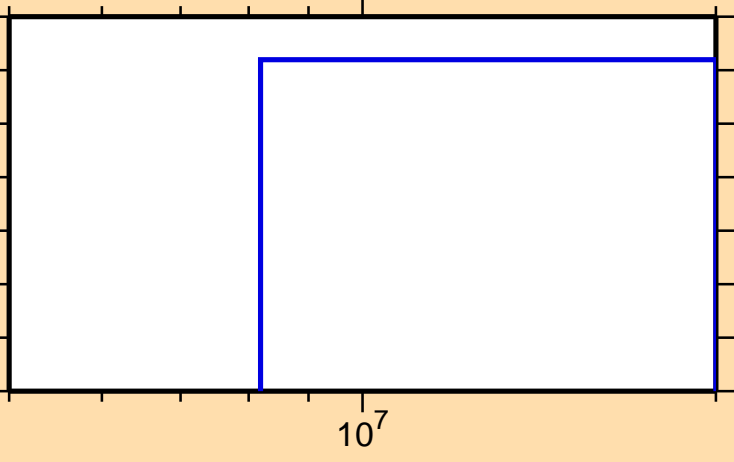
\sigma vs. E for ^{158}\text{Lu}(n,3n)
