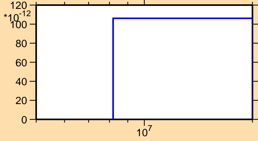
\sigma vs. E for ^{158}\text{Lu}(n,3n\alpha)
