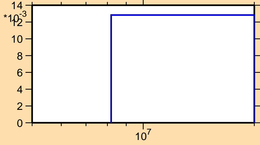
\sigma vs. E for ^{158}\text{Lu}(n,2n\alpha)
