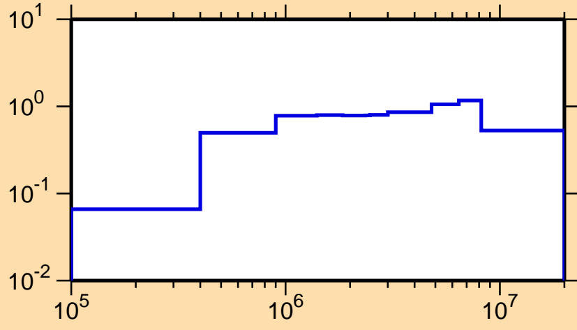
\sigma vs. E for ^{158}\text{Lu}(n,\text{inel.})
