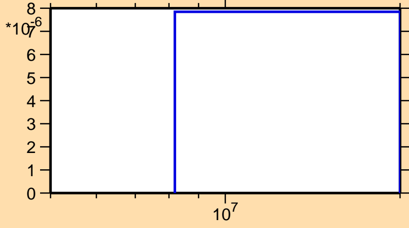
\sigma vs. E for ^{158}\text{Lu}(n,nd)
