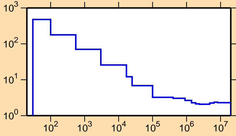
\sigma vs. E for ^{158}\text{Lu}(n,\text{nonel.})
