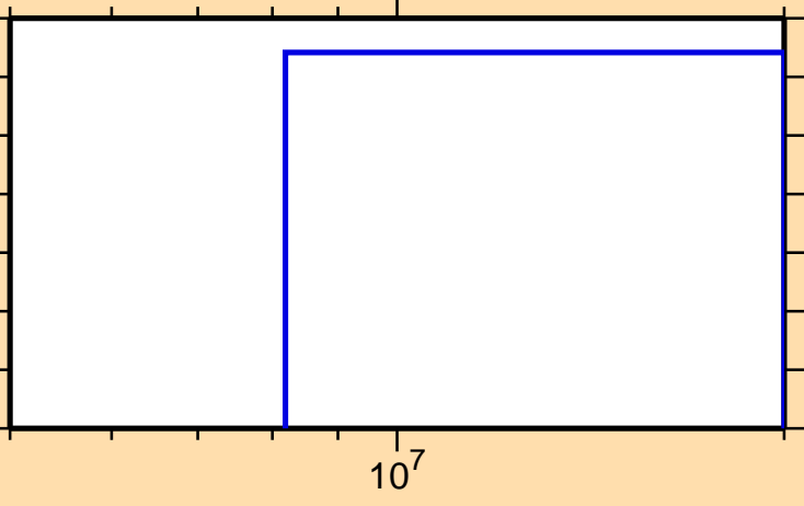
\sigma vs. E for ^{158}\text{Lu}(n,2n\alpha)
