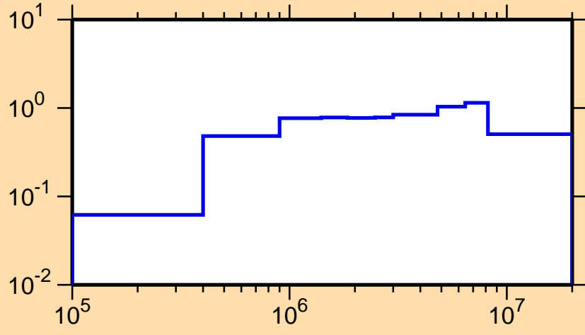
\sigma vs. E for ^{158}\text{Lu}(n,n\text{cont.})
