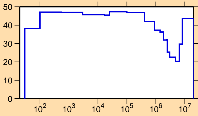
\Delta\sigma/\sigma vs. E for ^{158}\text{Lu}(n,p)
