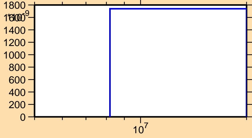
\sigma vs. E for ^{158}\text{Lu}(n,pd)
