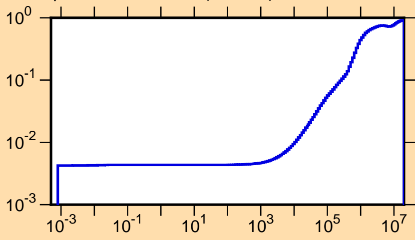
\mu vs. E for ^{159}\text{Lu}(\text{mt251})
