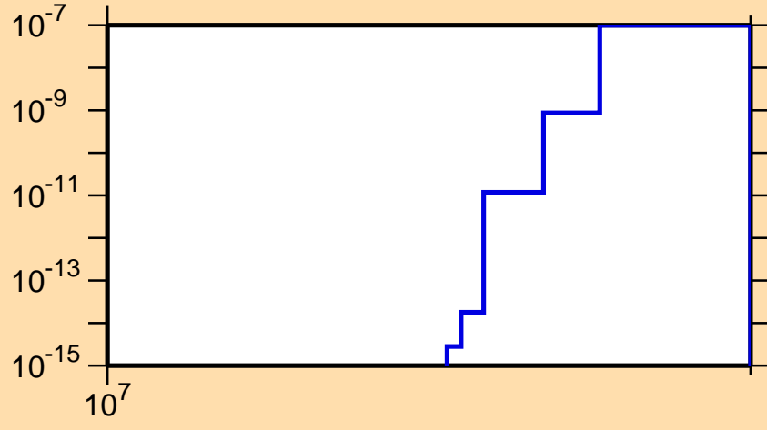
\sigma vs. E for ^{159}\text{Lu}(n,nt)
