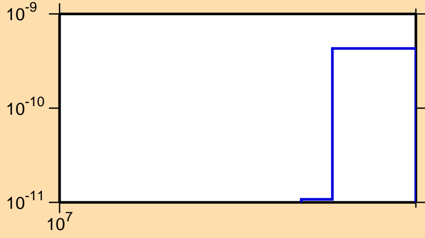
\sigma vs. E for ^{159}\text{Lu} (mt 34)
