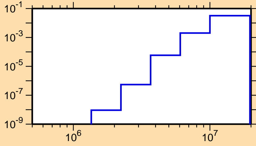
\sigma vs. E for ^{160}\text{Lu}(n,n\alpha)
