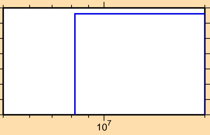
\sigma vs. E for ^{160}\text{Lu}(n,2np)
