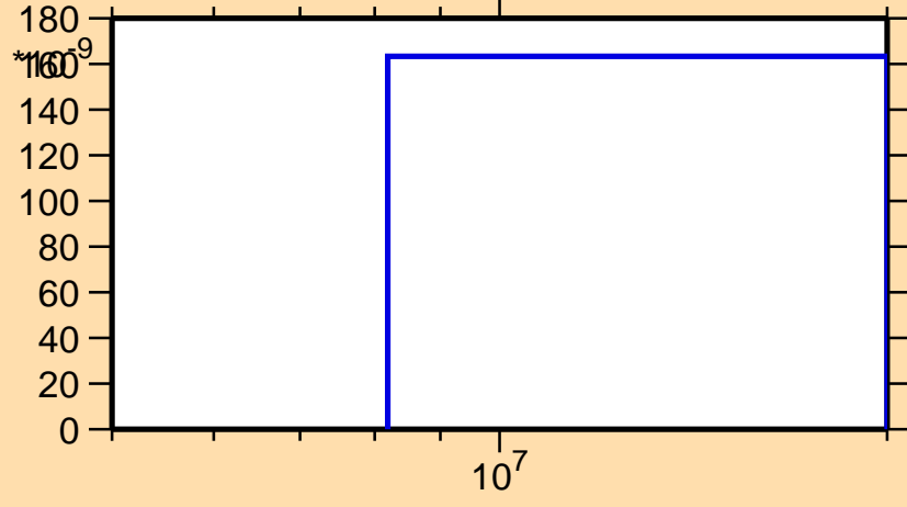
\sigma vs. E for ^{160}\text{Lu}(n,pd)
