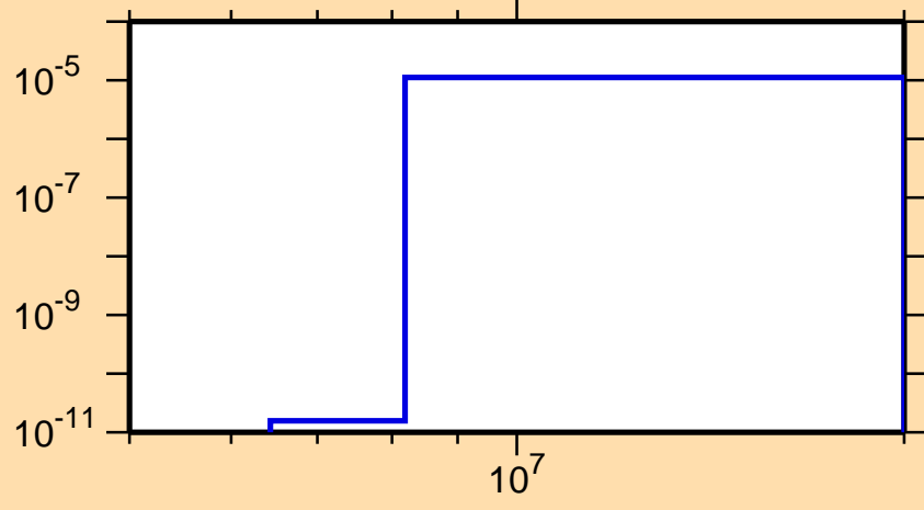
\sigma vs. E for ^{160}\text{Lu}(n,\text{He3})
