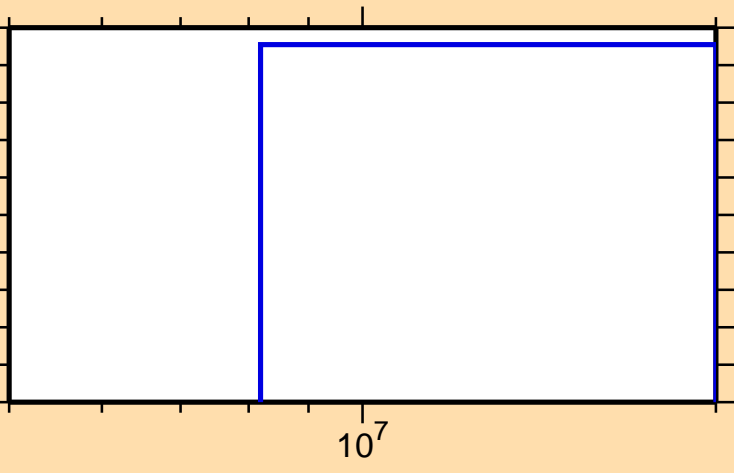
\sigma vs. E for ^{160}\text{Lu}(n,3n\alpha)
