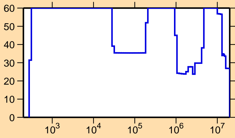
\Delta\sigma/\sigma vs. E for ^{160}\text{Lu}(n,el.)
