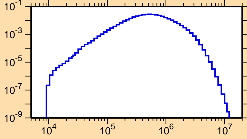
\sigma vs. E for ^{160}\text{Lu}(n,n_2)
