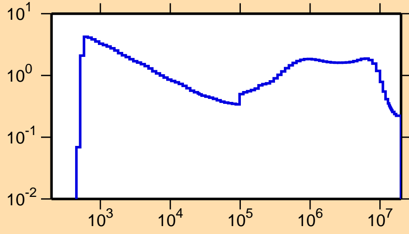
\sigma vs. E for ^{160}\text{Lu}(n,\text{inel.})
