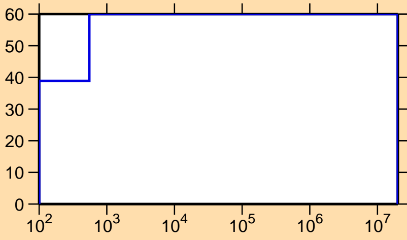
\Delta\sigma/\sigma vs. E for ^{160}\text{Lu}(n,\gamma)
