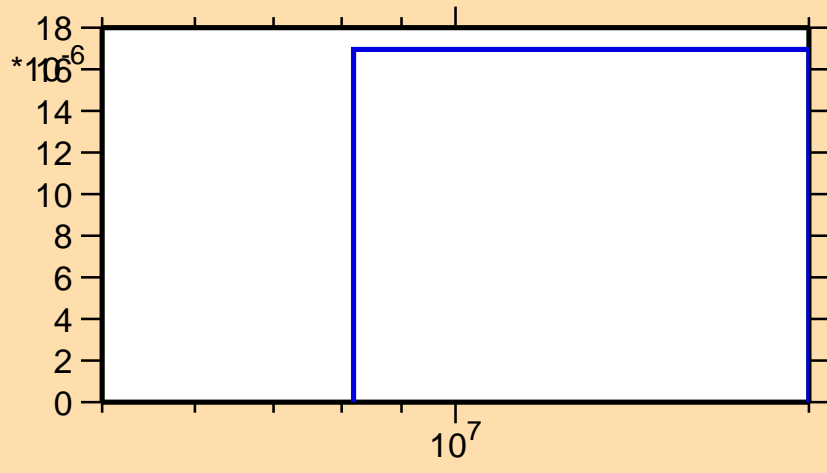
\sigma vs. E for ^{160}\text{Lu}(n,nd)
