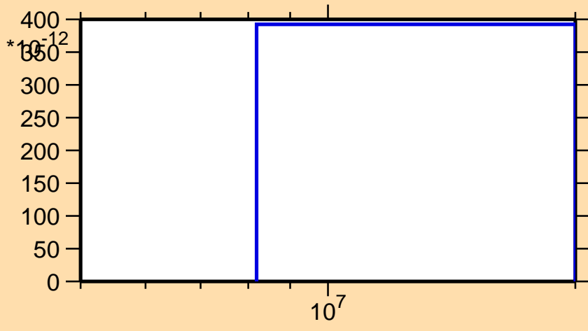
\sigma vs. E for ^{160}\text{Lu} (mt 34)
