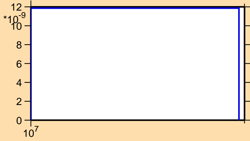
\sigma vs. E for ^{161}\text{Lu}(n,3n\alpha)
