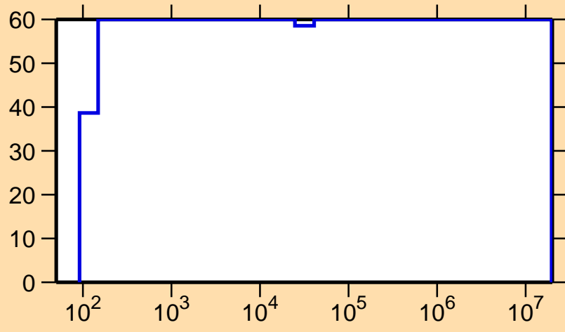
\Delta\sigma/\sigma vs. E for ^{161}\text{Lu}(n,p)
