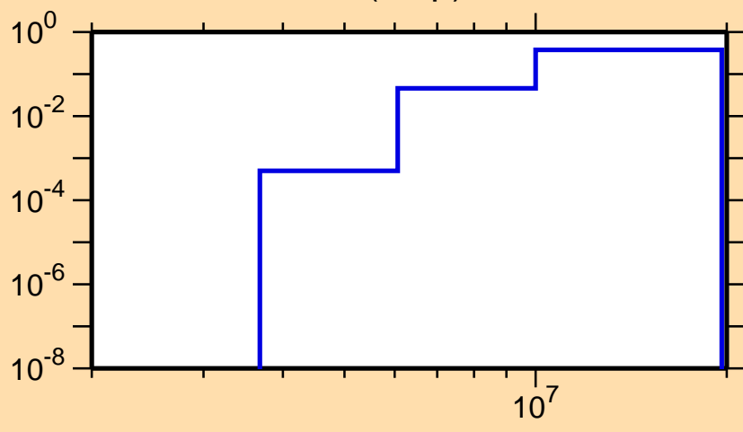
\sigma vs. E for ^{161}\text{Lu}(n,np)
