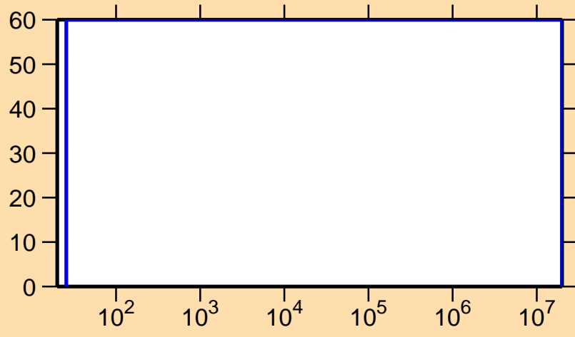
\Delta\sigma/\sigma vs. E for ^{162}\text{Lu}(n,\gamma)
