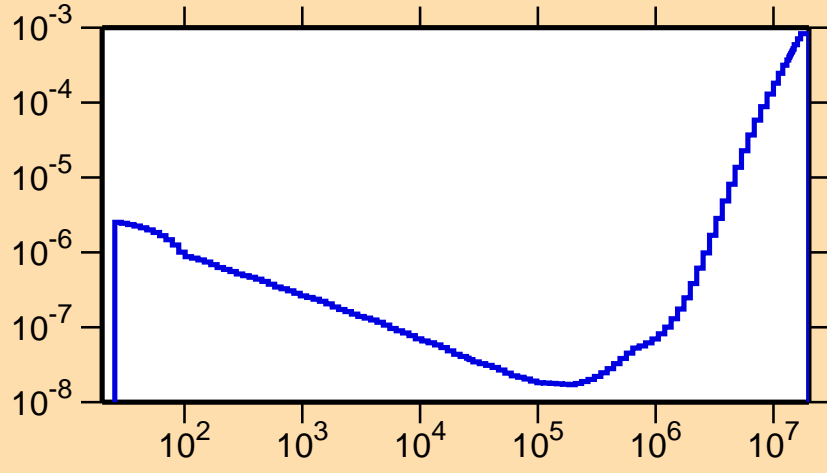
\sigma vs. E for ^{162}\text{Lu}(n,p\alpha)
