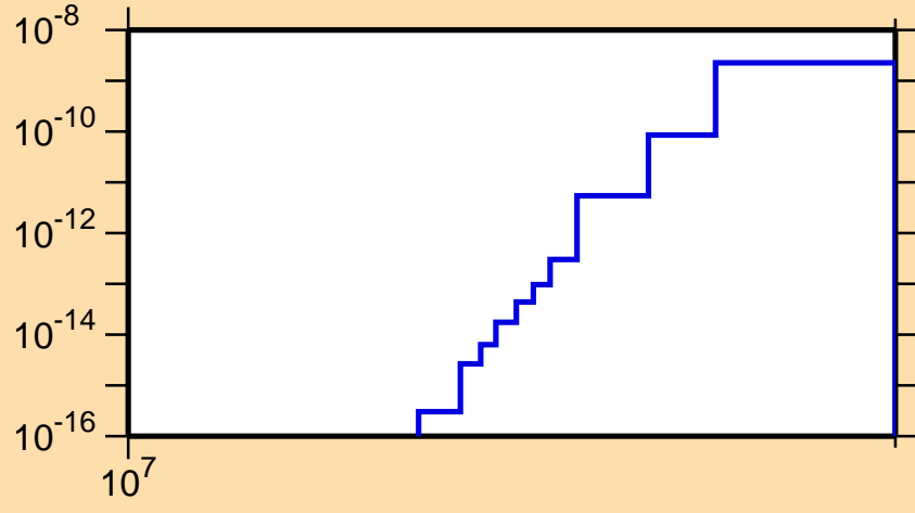
\sigma vs. E for ^{162}\text{Lu} (mt 34)
