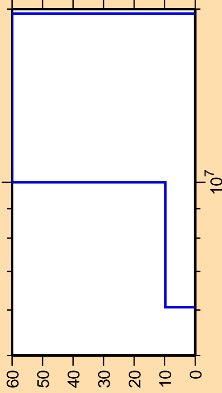
\Delta\sigma/\sigma vs. E for ^{162}\text{Lu} (mt 45)
