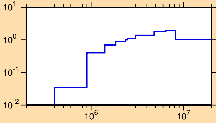
\sigma vs. E for ^{162}\text{Lu}(n,n\text{cont.})
