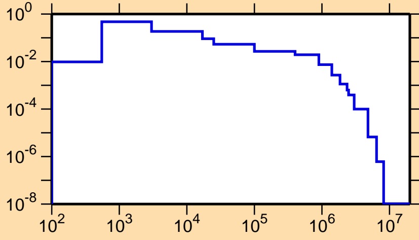
\sigma vs. E for ^{162}\text{Lu}(n,n_3)
