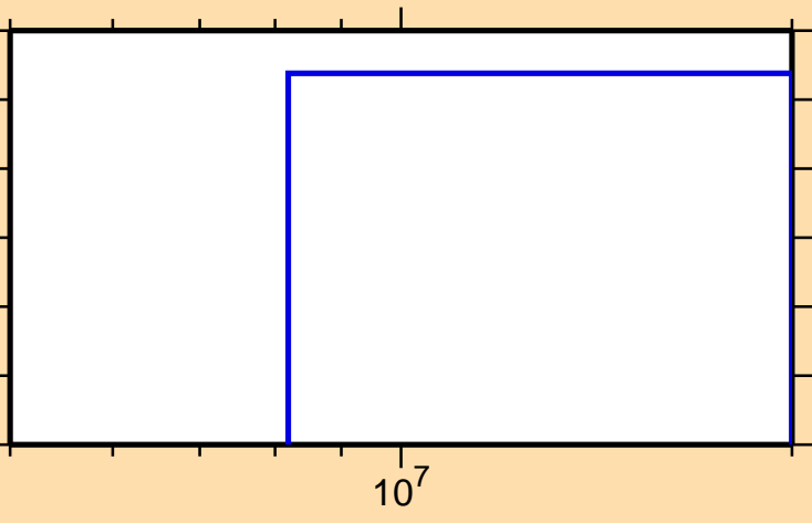
\sigma vs. E for ^{162}\text{Lu}(n,nt)
