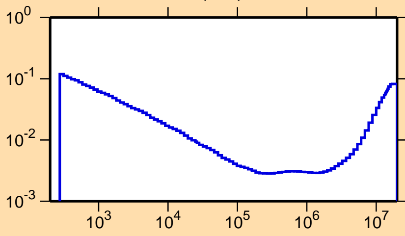
\sigma vs. E for ^{162}\text{Lu}(n,\alpha)
