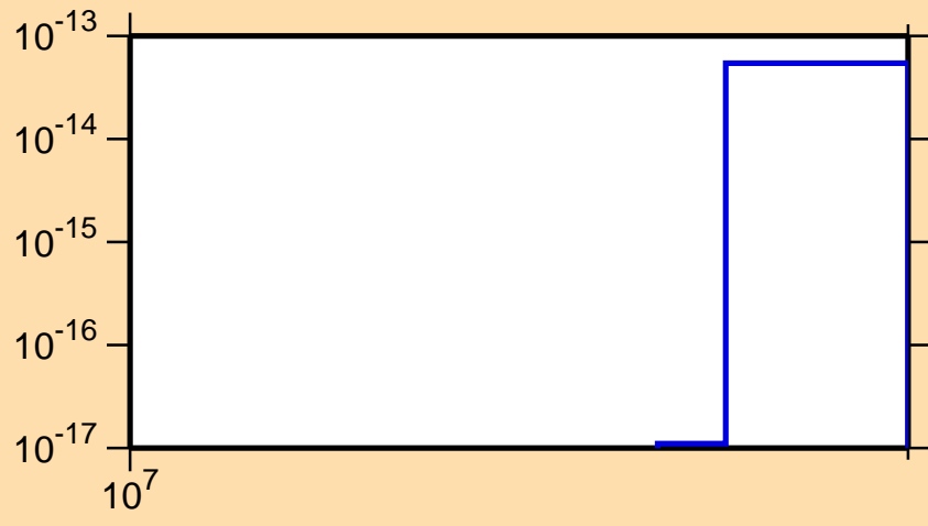
\sigma vs. E for ^{162}\text{Lu}(n,3n\alpha)
