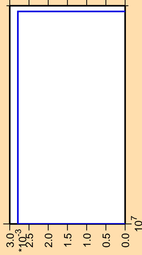
\Delta\sigma/\sigma vs. E for ^{162}\text{Lu}(n,3n\alpha)
