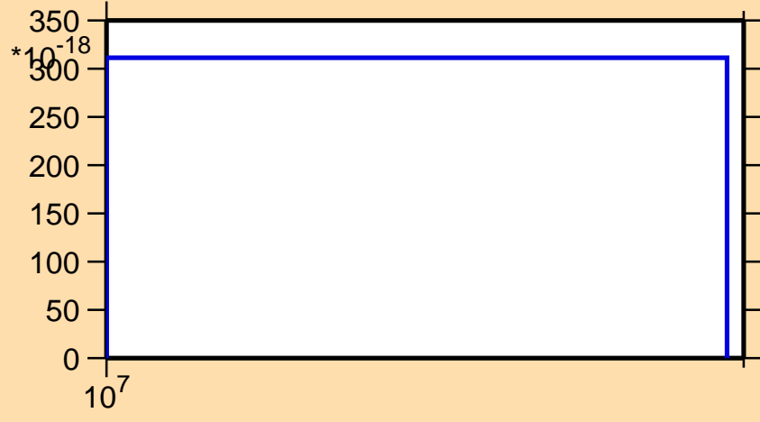
\sigma vs. E for ^{162}\text{Lu}(n,3n\alpha)
