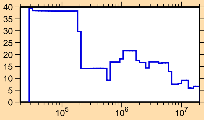
\Delta\sigma/\sigma vs. E for ^{164}\text{Lu}(n,\text{el.})
