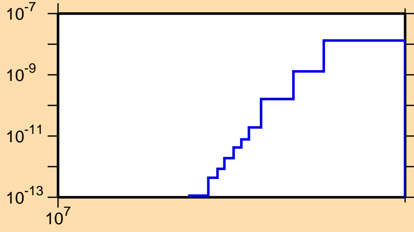
\sigma vs. E for ^{164}\text{Lu}(n,pd)
