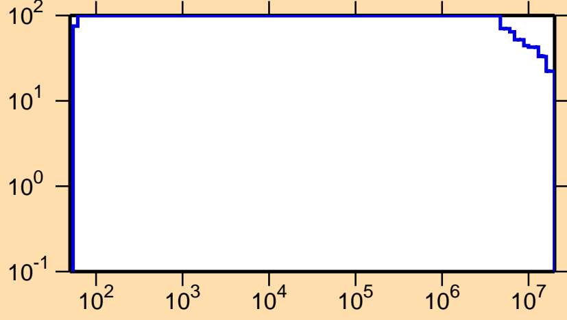
\Delta\sigma/\sigma vs. E for ^{164}\text{Lu}(n,p)
