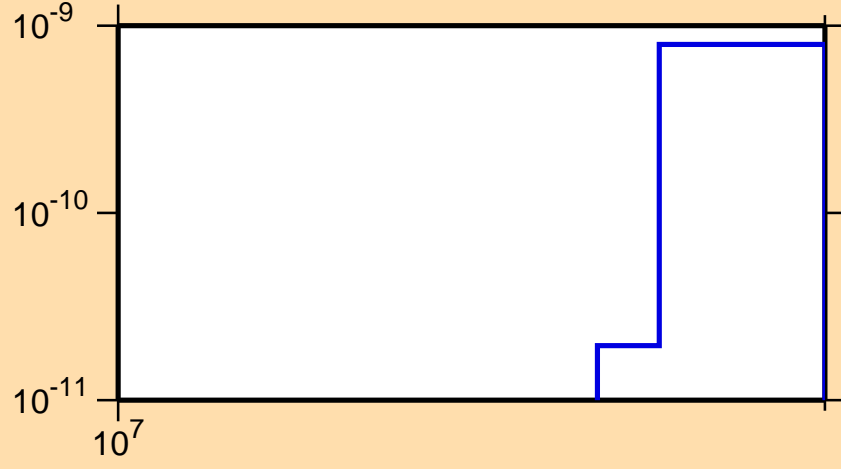
\sigma vs. E for ^{164}\text{Lu} (mt 34)
