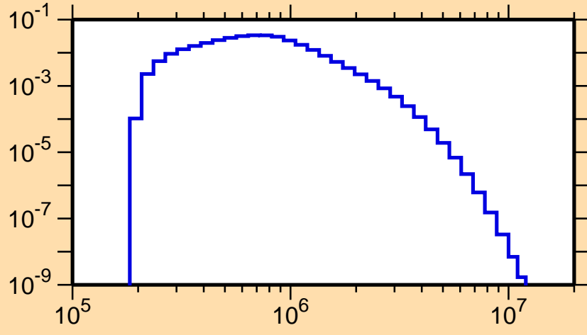
\sigma vs. E for ^{164}\text{Lu}(n,n_4)
