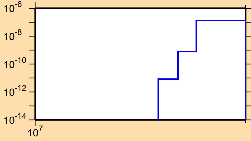
\sigma vs. E for ^{164}\text{Lu}(n,nt)
