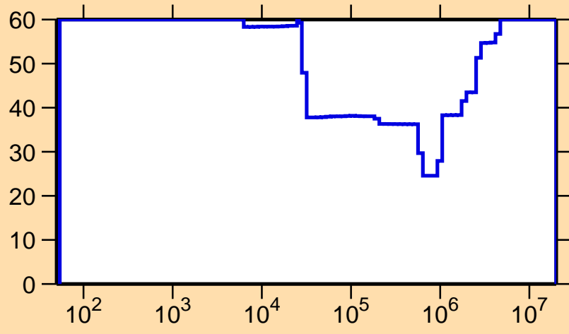
\Delta\sigma/\sigma vs. E for ^{164}\text{Lu}(n,\gamma)
