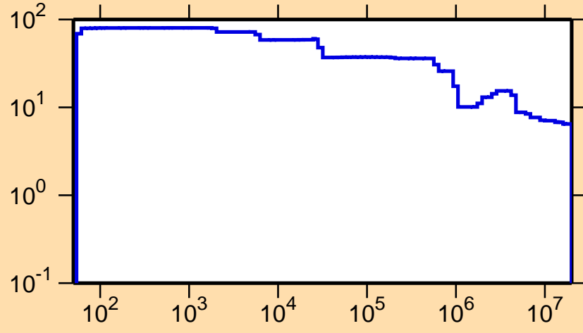
\Delta\sigma/\sigma vs. E for ^{164}\text{Lu}(n,\text{nonel.})
