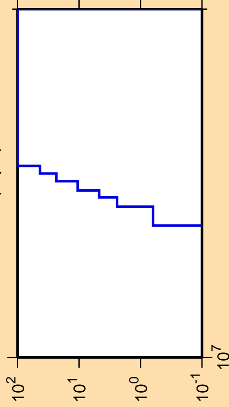
\Delta\sigma/\sigma vs. E for ^{164}\text{Lu}(n,pd)
