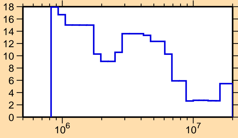
\Delta\sigma/\sigma vs. E for ^{164}\text{Lu}(n,\text{tot.})
