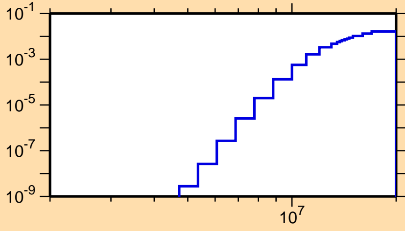
\sigma vs. E for ^{164}\text{Lu}(n,d)
