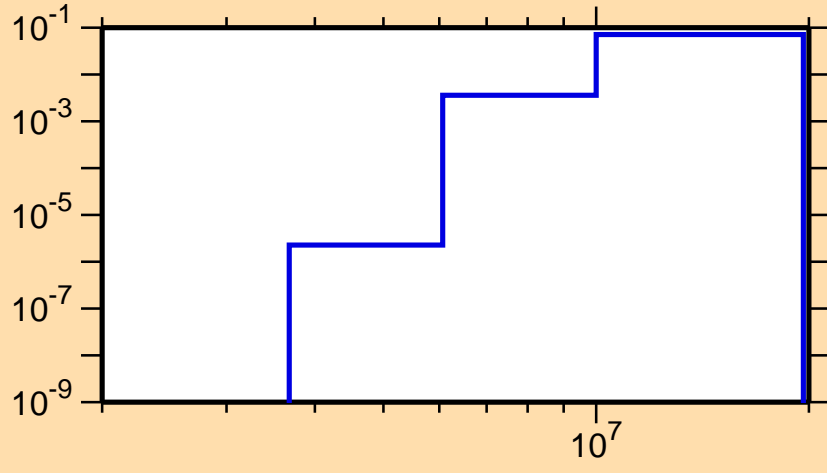
\sigma vs. E for ^{164}\text{Lu}(n,np)
