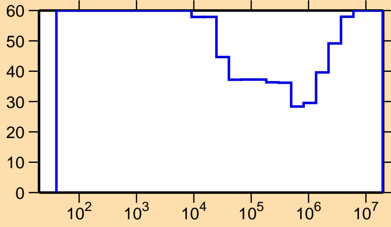
\Delta\sigma/\sigma vs. E for ^{164}\text{Lu}(n,\gamma)
