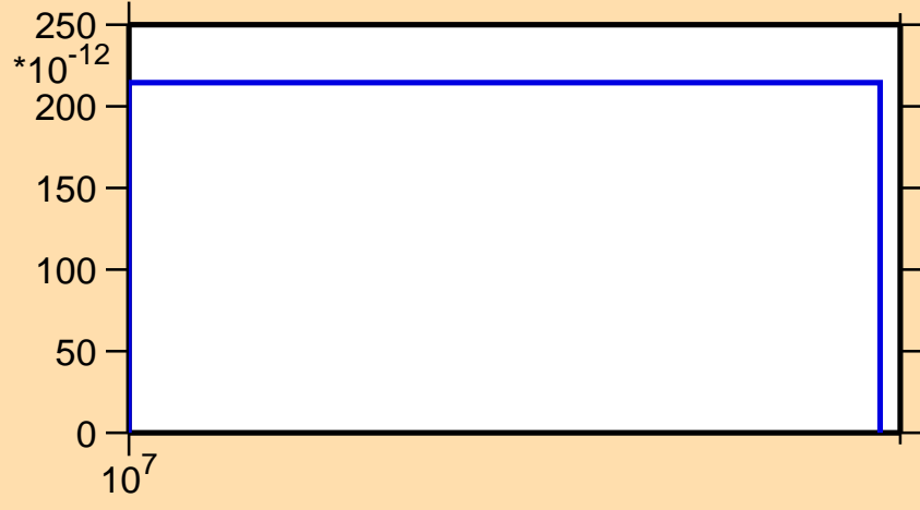
\sigma vs. E for ^{164}\text{Lu}(n,pd)
