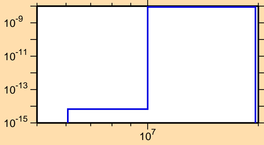
\sigma vs. E for ^{164}\text{Lu}(\text{mt117})
