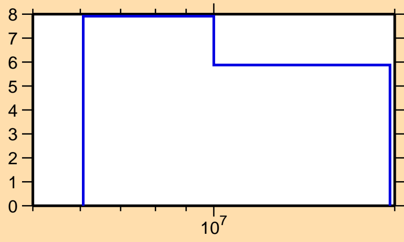
\Delta\sigma/\sigma vs. E for ^{164}\text{Lu}(n,\text{el.})
