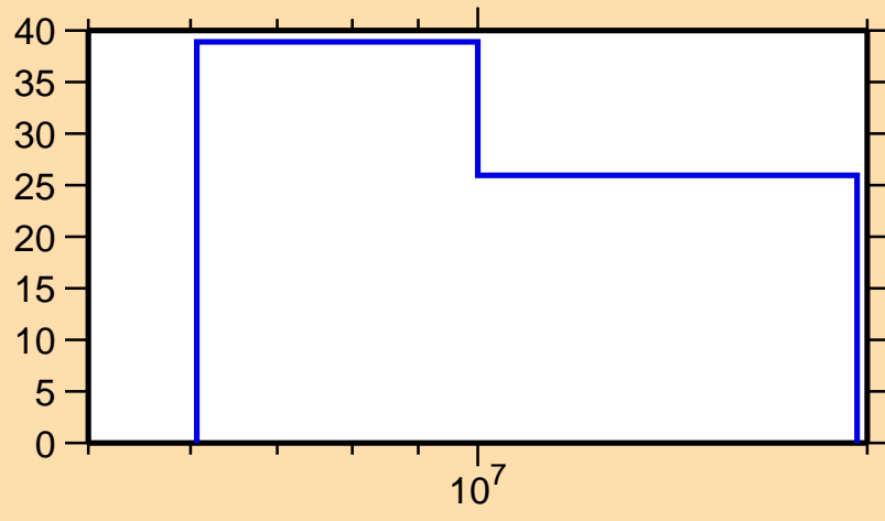
\Delta\sigma/\sigma vs. E for ^{164}\text{Lu}(n,2n)
