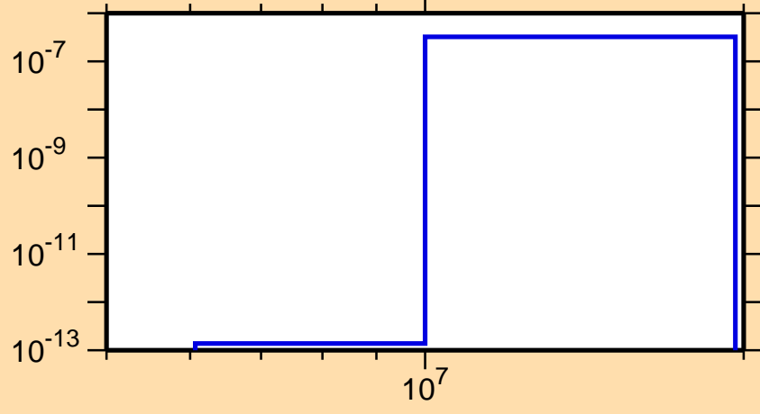
\sigma vs. E for ^{164}\text{Lu} (mt 45)
