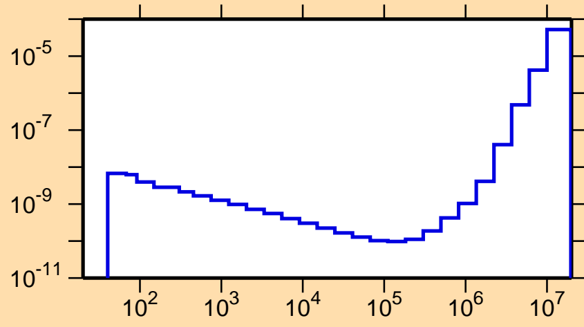
\sigma vs. E for ^{164}\text{Lu}(n,p\alpha)
