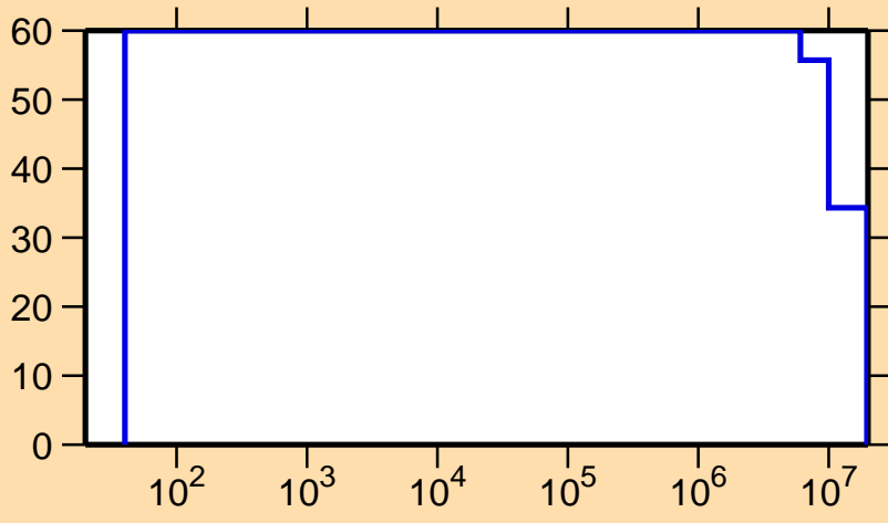
\Delta\sigma/\sigma vs. E for ^{164}\text{Lu}(n,p)
