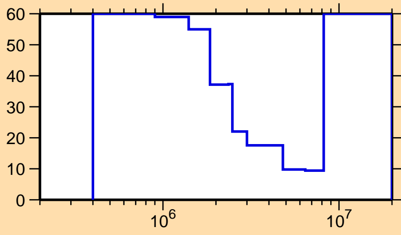
\Delta\sigma/\sigma vs. E for ^{164}\text{Lu}(n,n\text{cont.})
