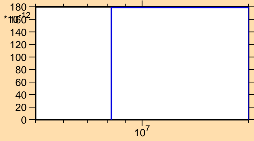
\sigma vs. E for ^{164}\text{Lu}(n,\text{pd})
