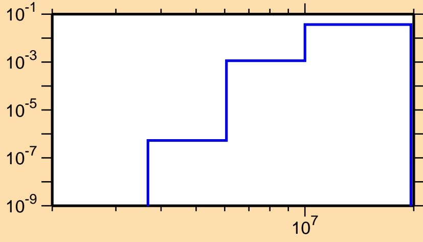
\sigma vs. E for ^{165}\text{Lu}(n,np)
