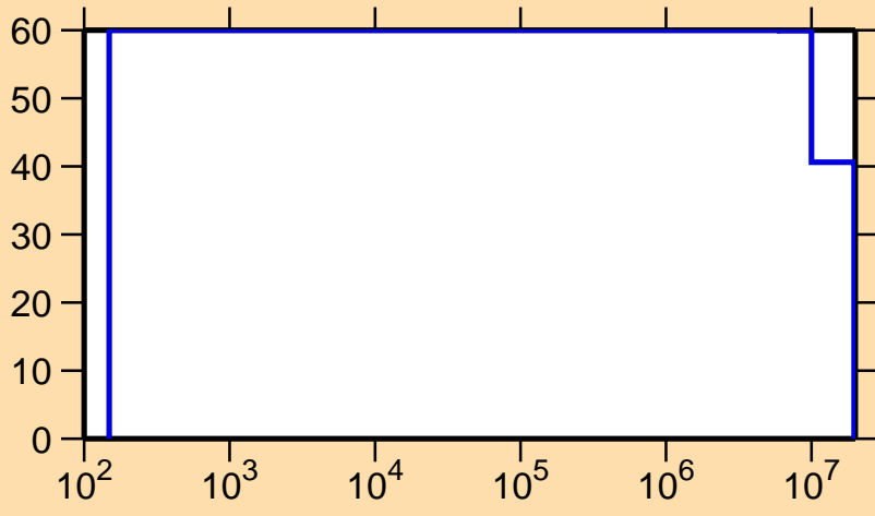
\Delta\sigma/\sigma vs. E for ^{165}\text{Lu}(n,p)
