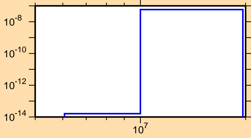
\sigma vs. E for ^{165}\text{Lu}(\text{mt } 45)
