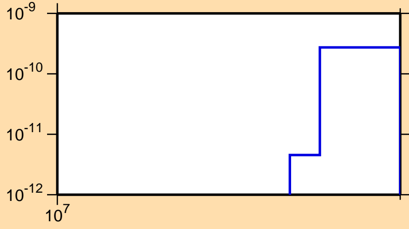
\sigma vs. E for ^{166}\text{Lu}(n,pt)
