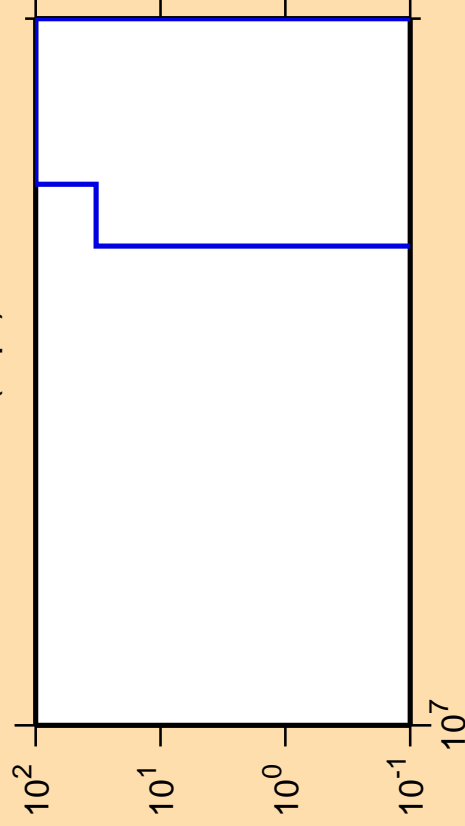
\Delta\sigma/\sigma vs. E for ^{166}\text{Lu}(n,pt)
